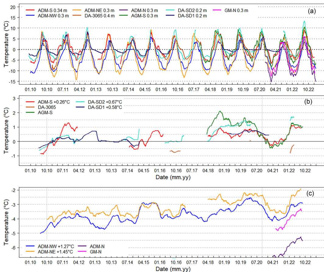
FIGURE 5 Near-surface temperature displayed with: (a) a 31-day running mean—depths of the near-surface sensors are given with the borehole names; (b, c): a 365-day running mean (linear trends over the reference decade are given in the keys, vertical dotted lines delineate the decade). [Colour figure can be viewed at wileyonlinelibrary.com ]
