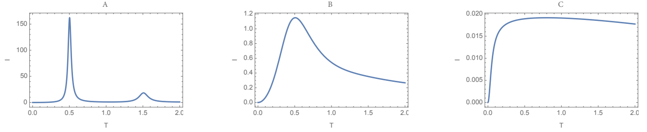
FIG. 2. Value of the dimensionless thrust as function of the period T , for various values of \xi : a) \xi = 0.1 . b) \xi = 1.2 . c) \xi = 10
