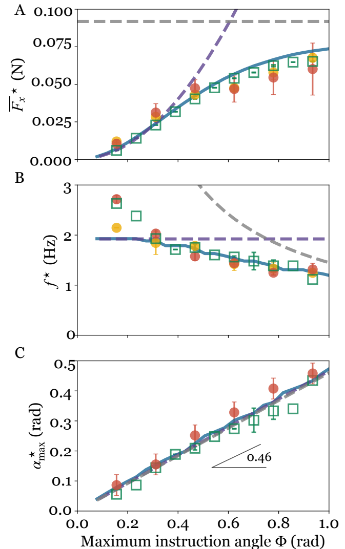
FIG. 3. (A) Maximum average thrust \bar{F}_x^* . (B) Optimal undulation frequency f^* . (C) Maximal fin angle \alpha_{\max}^* . For each figure, we compare the experimental results and those obtained with the model (Eqs. 1, 2 and 3). Experimental results: the red symbols are obtained via RL with the state (F_y, \dot{F}_y, \phi_c) ; the orange symbols are obtained via image learning, where the state is a set of four successive pictures of the robot. Simulation results: the open square symbols denote RL results with the simulation of the model. The dashed violet and gray curves represent theoretically predicted values in the limits of very small and very large \Phi , respectively. The solid green curve corresponds to the numerical determination of the frequency f^* that yields the highest thrust, F_x^* , assuming a square waveform for \phi_c .
