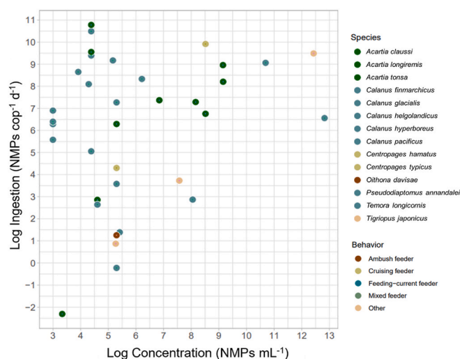
Fig. 7. Microplastic ingestion (NMPs \text{cop}^{-1} \text{d}^{-1} ) by all copepod species studied in this review exposed to different plastic concentrations (NMPs \text{mL}^{-1} ). Copepod species are grouped by color based on their foraging behavior. Note: Ingestion or concentration maximum average was represented when maximum overall value was not provided.
