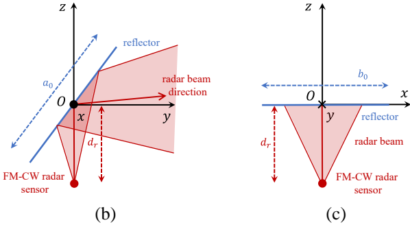
Fig. 1. (a) Annotated photo of the mm-wave FM-CW radar system used to track small moving targets in the 3D space. The Cartesian ( x , y and z ) coordinate system and the origin set on the rotating axis centered with the radar front-end are shown. Schematic representation of the beam scanning system projected on (b) Oyz plane and (c) Oxz plane ( a_0=20\text{cm} and b_0=25\text{cm} are respectively the width and length of the rectangular plate used as a reflector).
