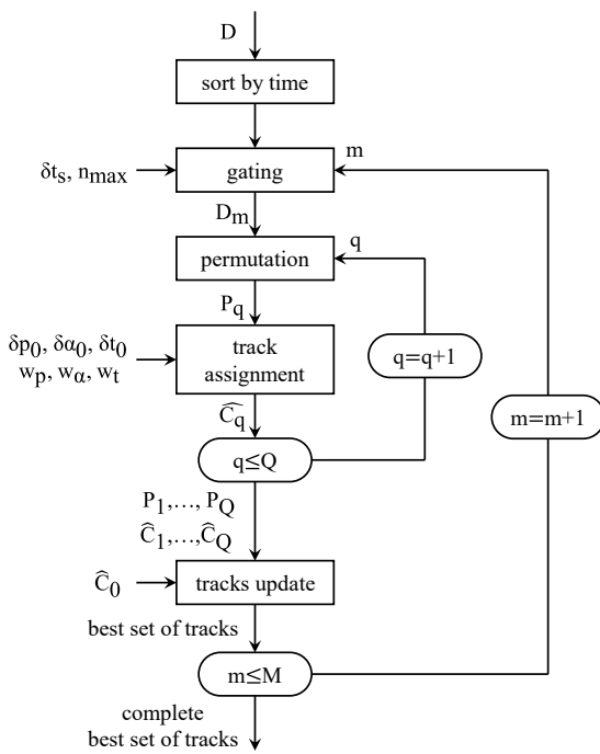
Fig. 2. Flowchart of the MT 2 algorithm from the detection set to the selected tracks (i.e., the complete best set of tracks) for a given (forward or backward) reconstruction method.
