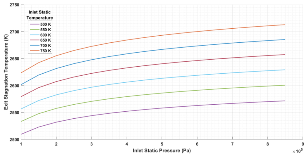
Fig. 12 RDE combustor temperature map for equivalence ratio 1 and exit Mach number 0.8.
