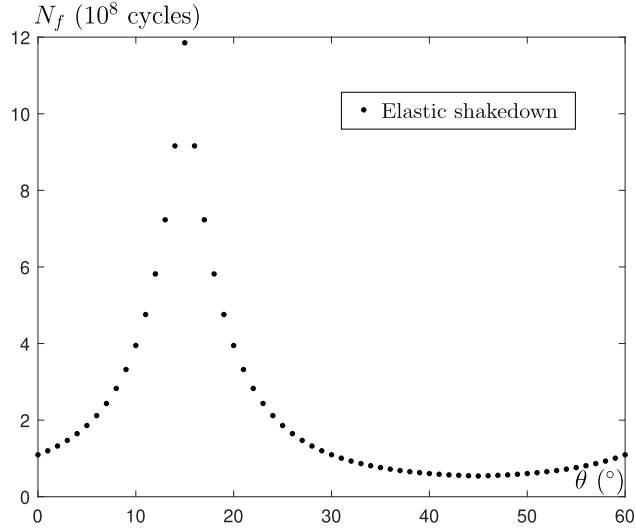
Figure 10: Fatigue lifetime N_f as a function of crystal orientation \theta^\circ for condition 1.
