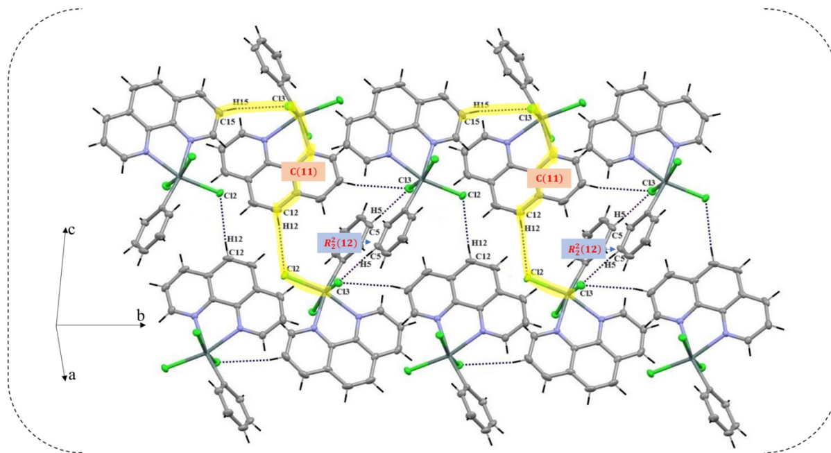
Figure 3 Intermolecular hydrogen bonds: C15-H15\cdots Cl3^i , C5-H5\cdots Cl3^{ii} , and C12-H12\cdots Cl2^v and hydrogen-bonded planes in the title compound. [Symmetry codes: (i) -x + \frac{3}{2}, y + \frac{1}{2}, -z + \frac{3}{2} ; (ii) -x + 1, -y + 1, -z + 2 ; (v) x + \frac{1}{2}, -y + \frac{3}{2}, z - \frac{1}{2} ]
