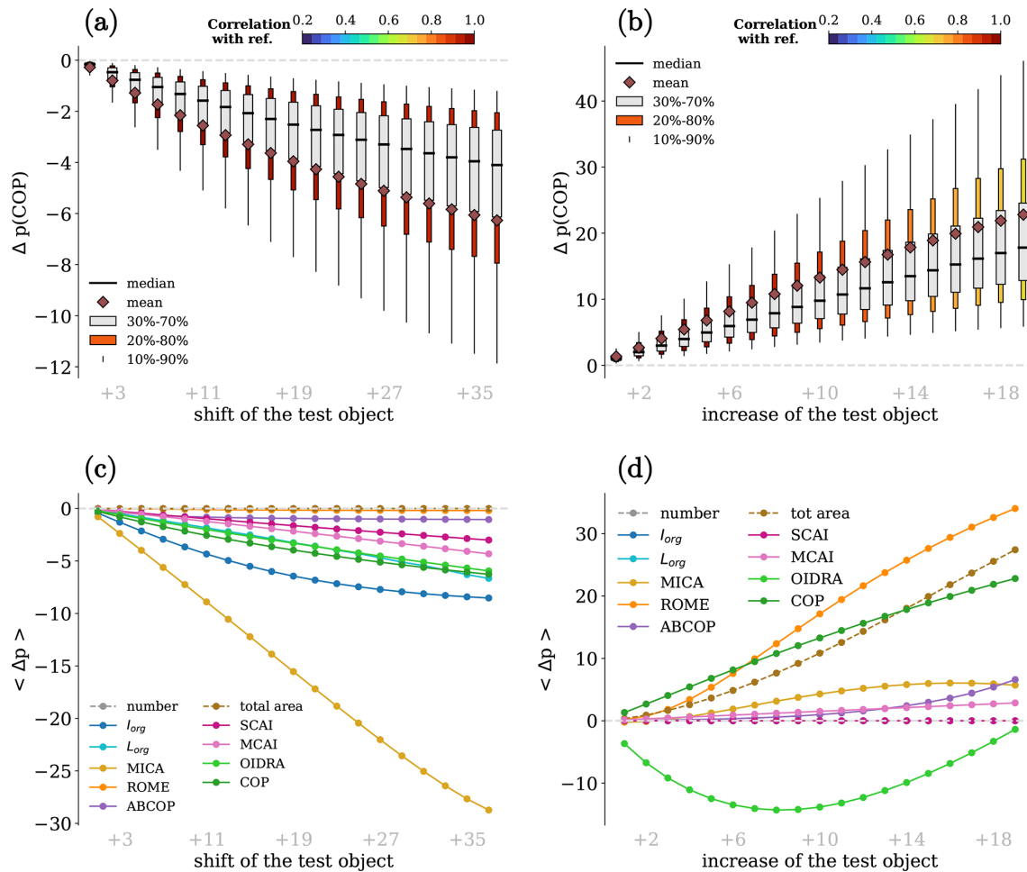
Figure 7. Distribution of \Delta p(\text{COP}) as a function of perturbation (3) (a) and perturbation (4) (b). The gray boxes indicate the percentile range from 30% to 70%, the colored boxes indicate the percentile range from 20% to 80%, and the colors display the correlation between the reference and the modified dataset. The whiskers cover 10% to 90% of the distributions. The means and the medians of \Delta p(\text{COP}) are shown by the rhombuses and the black lines, respectively. The means of \Delta p are displayed for all the indices as a function of the perturbations of condition (3) (c) and condition (4) (d).
