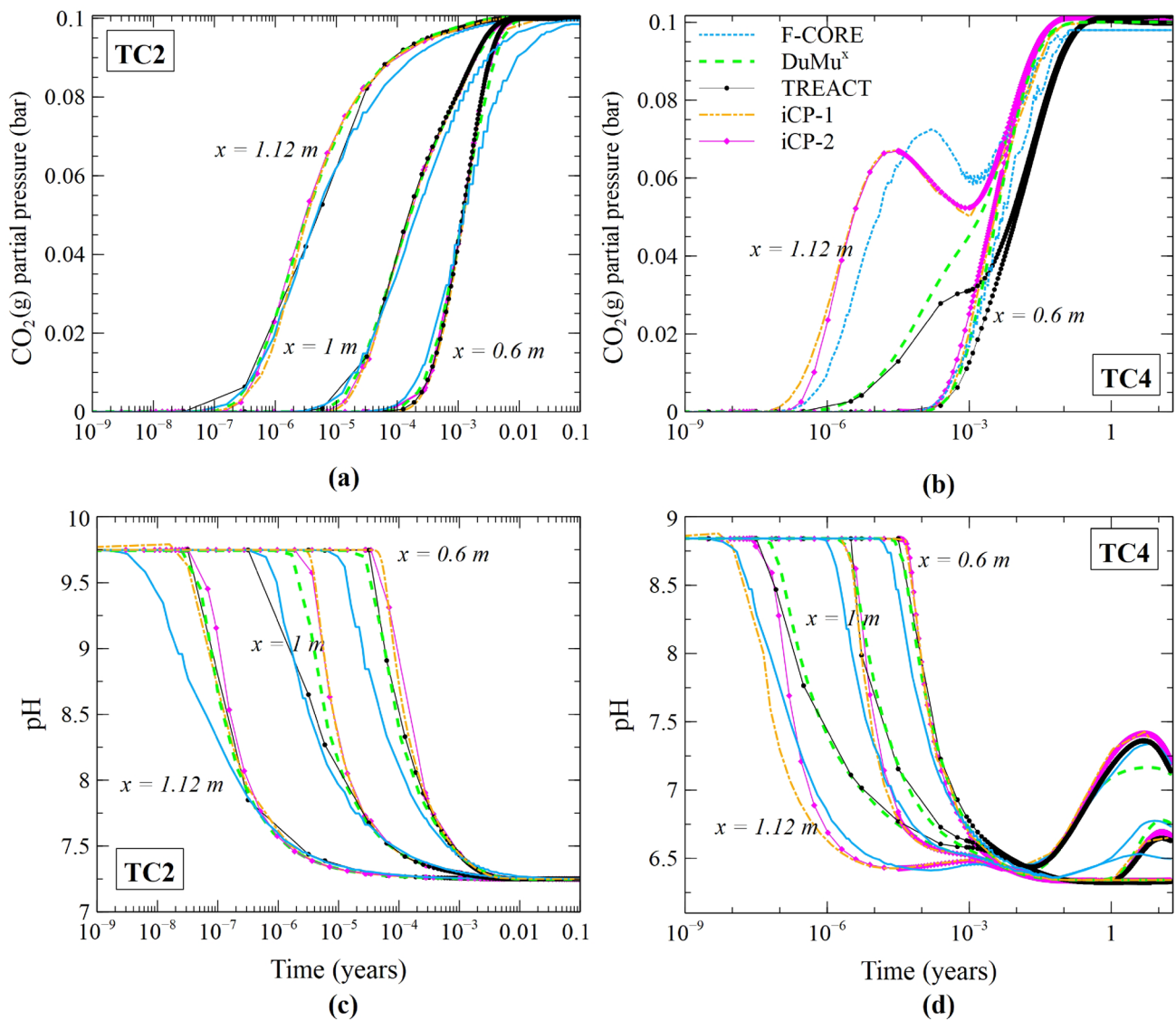
Fig. 4 Benchmarking of the time evolution of computed: a Partial pressure of \text{CO}_{2(g)} for case TC2 at x = 1.12\text{ m} , 1\text{ m} and 0.6\text{ m} ; b Partial pressure of \text{CO}_{2(g)} for case TC4 at x = 1.12\text{ m} and 0.6\text{ m} ; c pH for
