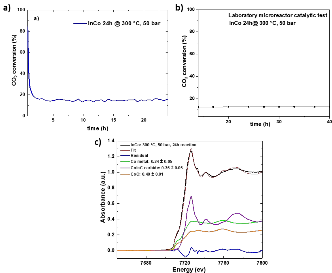
Figure 5: a) Evolution of the CO 2 conversion as function of time at 300 °C and 50 bar in the high-pressure/high-temperature reaction cell b) Evolution of the CO 2 conversion as function of time at 300 °C and 50 bar in the laboratory microreactor conditions c) Co K-edge XANES spectra at 300 °C and 50 bar and LCF of the XANES spectra of InCo catalysts after 24h of CO 2 hydrogenation reaction (final state)
