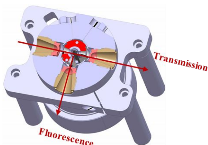
Figure 2. 3D representation of the general geometry of Beryllium windows in the high-pressure/high-temperature reaction cell, illustrating two windows along the beam axis for spectrum collection in transmission mode, and a third window positioned at a 90° angle to the beam for spectrum collection in fluorescence mode.
