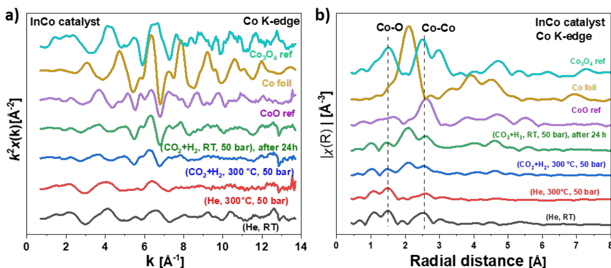
Figure 6. a) Co K-edge EXAFS k^2 \cdot \chi(k) functions of the InCo catalyst at different cycle of the \text{CO}_2 hydrogenation reaction, compared to those of the Co foil, CoO and \text{Co}_3\text{O}_4 reference compounds. b) The corresponded Co K-edge operando FT-EXAFS spectra.
