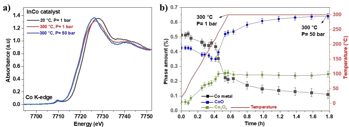
Figure 4: Heating and pressurization of the InCo catalyst under Helium a) Co K-edge XANES spectra of InCo catalyst under He at initial state (20 °C), after heating to 300 °C and then after pressurization to 50 bar at 300 °C b) phase amount of Co species during the thermal treatment of the InCo catalyst under He up to 300 °C and pressurization up to 50 bars under He.
