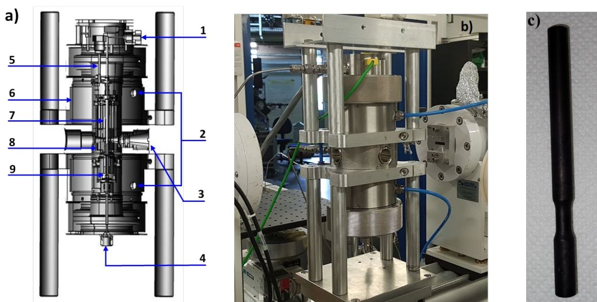
Figure 1. (a) 3D layout of the reaction cell set-up: (1) inlet of the gases to the cell, (2) plugs for cooling water circulation, (3) One of three windows, (4) gas outlet, (5) thermocouple to the heating system, (6) He inlet, (7) glassy carbon tube, (8) heating elements, (9) Region of mixture of gas products and He; (b) Real view of the fully assembled HP/HT cell in the SAMBA beamline at SOLEIL Synchrotron ready for operation; (c) Glassy carbon reactor machined at 350 \mu\text{m} thickness wall at the window zone.
