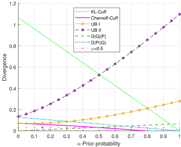
Fig. 2. Numerical comparison of different upper bounds on C(P, Q) derived through \epsilon -DP, KL-DP and Bhattacharya-DP which is C(P, Q) with \alpha = .5 .
