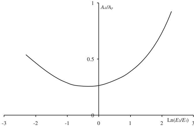
Fig. 10.11. Dimensionless ratio A_d/A_p vs. ratio of Young's moduli for two adjacent materials for a doubly symmetric deflection.
