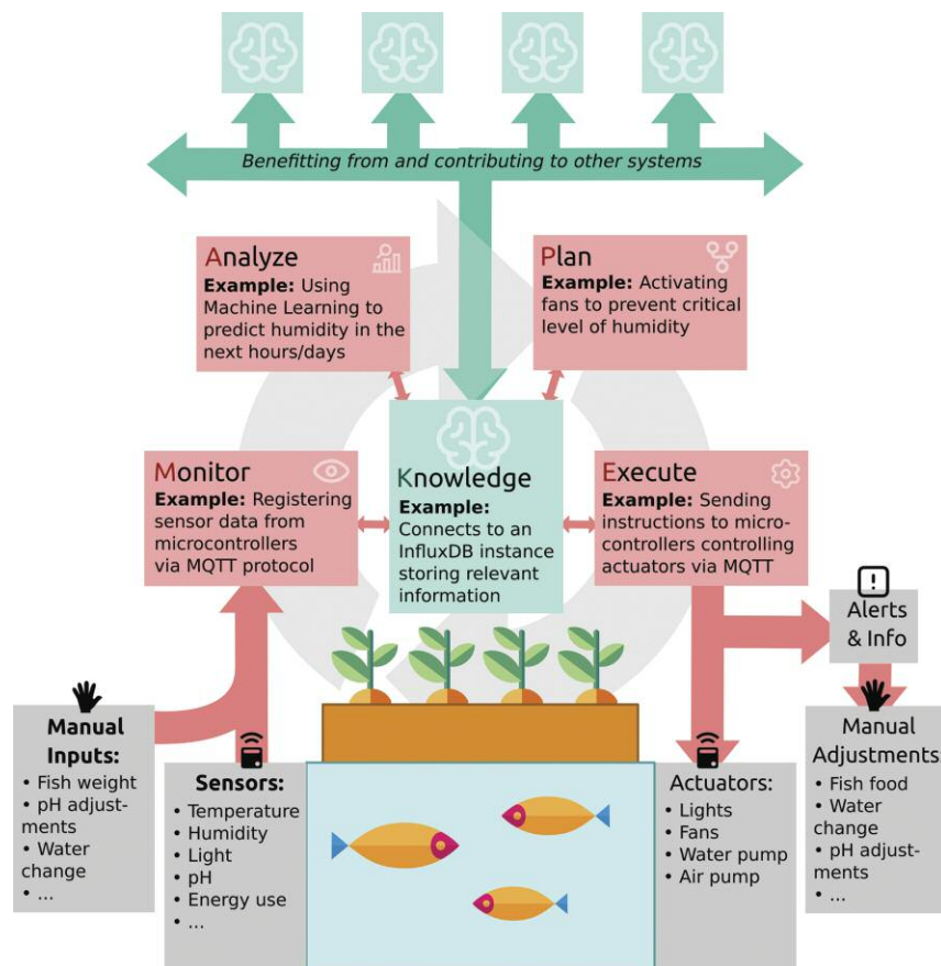
Figure 1: MAPE-K framework architecture for smart control of an aquaponics system.
