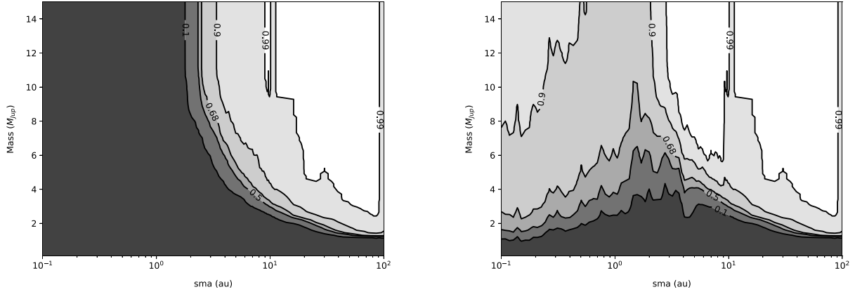
Fig. 18. Detection maps using the MESS2 (Lannier 2015) tool for HD 22917, DI only (left), DI+RV (right). The eccentricity is assumed between 0 and 0.5 and the inclination between 0 and 90 degrees. Contrast maps are converted to mass maps using the COND atmospheric model (Allard et al. 2001) and the stellar parameters of the system are extracted from Desidera et al. (2021). Two epochs were used here.
