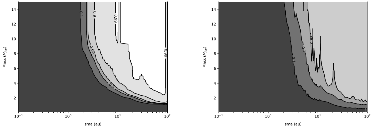
Fig. 19. Comparison between the detection limits obtained with PACO ASDI (left) and TLOCI (right) for HD 22917 using the MESS2 tool (Lannier 2015). The eccentricity is assumed between 0 and 0.5 and the inclination between 0 and 90 degrees. Contrast maps are converted to mass maps using the COND atmospheric model (Allard et al. 2001) and the stellar parameters of the system are extracted from Desidera et al. (2021). Two epochs were used.
