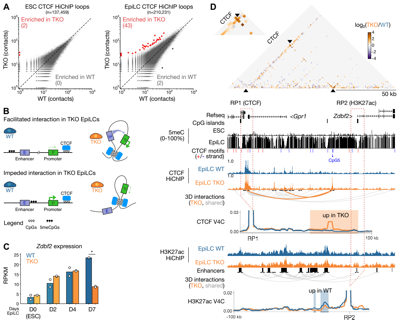
Figure 3. A subset of CTCF loops and promoter-enhancer contacts are disrupted in 5meC-deficient EpiLCs. (A) 2D scatterplots of CTCF loop contacts in WT versus TKO ESCs (left) and EpiLCs (right). Loops with significantly enriched contacts in TKO cells (FDR < 0.05) are highlighted in red. (B) Schema showing two potential scenarios resulting from global DNA hypomethylation in TKO EpiLCs (right) due to CTCF binding and altered promoter-enhancer contact formation and nearby gene transcription. Top: a hypomethylated CTCF binding site creates a loop that increases enhancer-promoter interactions. Bottom: a hypomethylated CTCF binding site results in a loop that insulates enhancer-promoter interactions. (C) Bar plot of Zdbf2 expression levels (RPKM) in a time course assay of ESC-to-EpiLC differentiation in WT and TKO cells. Bars represent the mean, and replicates are shown as dots. D: days EpiLC differentiation. Statistically significant changes in gene expression between WT and TKO (Linear modeling with Limma, fold-change > 1, t-test adjusted P value < 0.05) are indicated by asterisks. (D) Contact matrix (top), genome browser screenshot (middle) and virtual 4C (bottom) plots of the Zdbf2 locus. Top: differential CTCF contacts between WT and TKO EpiLCs are displayed, where each pixel represents a 1 kb bin. The TKO-enriched contacts between the TAD border and the putative 5meC-sensitive CTCF binding site is magnified in the inset. Reference points 1 (CTCF) and 2 (H3K27ac) for the virtual 4C plots (bottom) are indicated by a dashed box. Middle: browser screenshot showing CpG methylation, CTCF and H3K27ac enrichment levels and loops. Gray loops represent significant interactions that are consistent across the data being compared, orange loops are TKO-specific. Refseq genes, CpG islands, CTCF motifs (positive strand in red, negative strand in blue) are included. The CTCF motif with a CpG at position 5 that underlies a putative 5meC-sensitive CTCF peak is highlighted. Bottom: Virtual 4C plots of reference points 1 (CTCF) and 2 (H3K27ac) showing interaction frequencies between the reference point and adjacent area. The background model is shown as a dotted gray line. Statistically enriched contacts (chi-squared test, alpha < 0.25) are highlighted in blue (WT EpiLC-specific) or orange (TKO EpiLC-specific). Coordinates: chr1:63165972–63304123.
