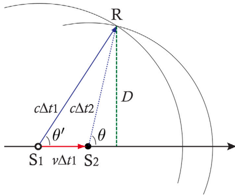
Fig. 5. Two successive pulses are sent to the receptor, with the second pulse being sent exactly when the first is received.
