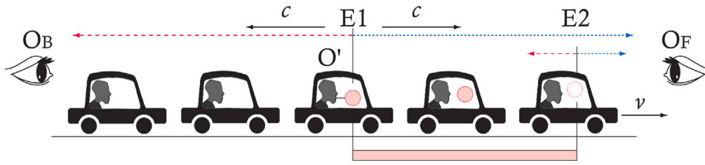
Fig. 1. Events of birth ( E1 ) and disappearance ( E2 ) of a soap bubble in a vehicle moving at constant speed v with respect to observers, one located at the back ( O_B ) and the other at the front ( O_F ) of the vehicle. The images of the formation and the bursting of the bubble reach the observers at the speed of light c .
