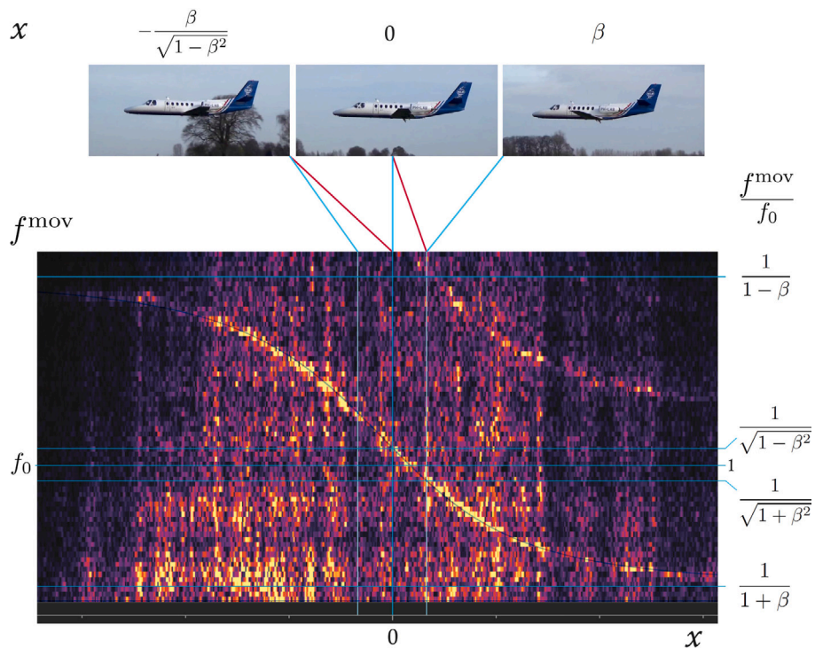
Fig. A.1. Doppler effect illustrated by a dominant frequency recorded during the passage of an airplane at low altitude. The blue lines connecting the images of the planes to the spectrogram indicate the actual coincidence of sound and image on the film, while the red lines connect the recorded frequencies to their actual points of emission. (For interpretation of the references to color in this figure legend, the reader is referred to the web version of this article.)
