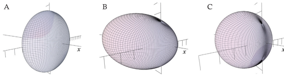
Fig. 3. Perspective view of the shapes of (A) the material sphere drawn to Eq. (23), (B) the received relativistic wavefront surface drawn to Eq. (27) and (C) the Galilean wavefront drawn to Eq. (30), for \beta = 0.9 . In the wavefront panels B and C, the source is located at the intersection of the axes.
