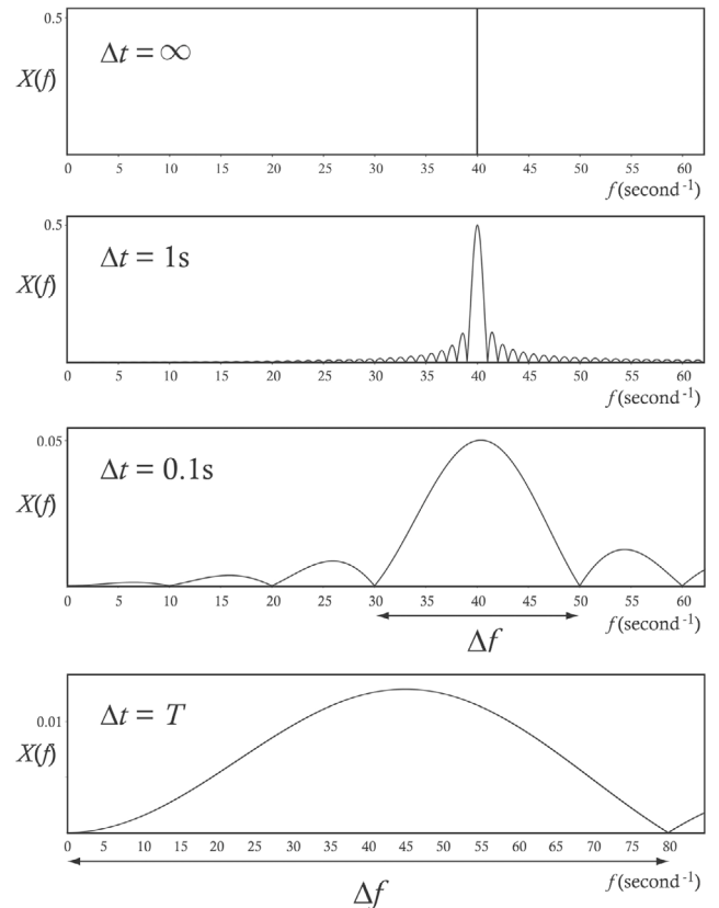
Fig. 6. Increasing imprecision in frequency as the duration of the signal decreases. Example of a sound of 40 Hertz (40 cycles per second). An infinite (non-physical) duration of the sound allows the absolute focusing of its frequency (top panel). We observe a broadening of the frequency peak ( \Delta f ) and the appearance of parasite frequencies as the signal duration ( \Delta t ) is shortened.
