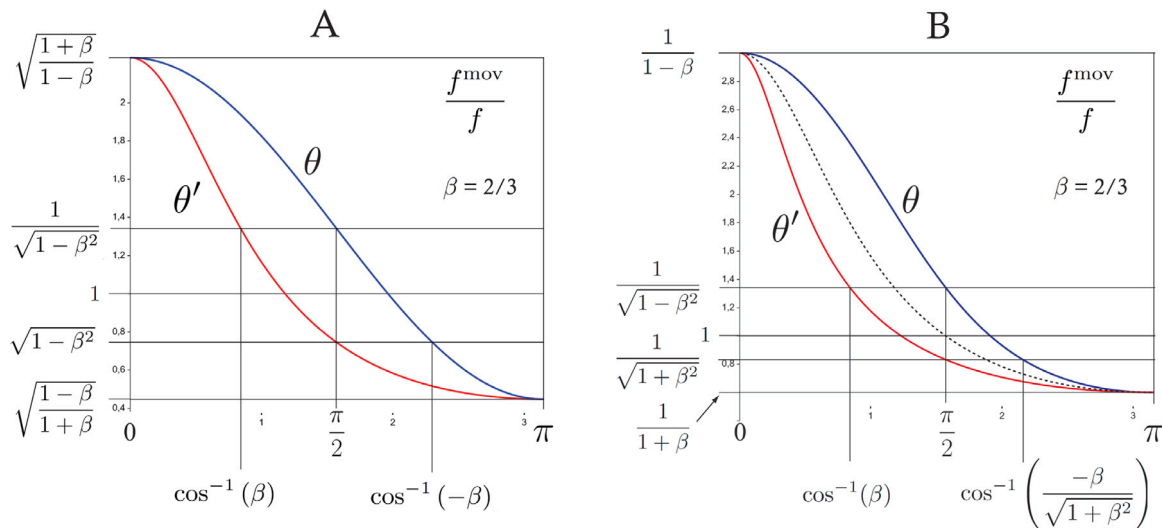
Fig. 4. Doppler effects as functions of the angles \theta and \theta' . Since the true determinants of energies and colors are frequencies, Doppler effects are described in terms frequency ratios. (A) Relativistic Doppler effect deduced from the perceived ellipsoidal wavefront. (B) Galilean Doppler effect derived from the perceived spherical wavefront. The dashed black curve corresponds to the so-called classical Doppler effect, shown for comparison.
