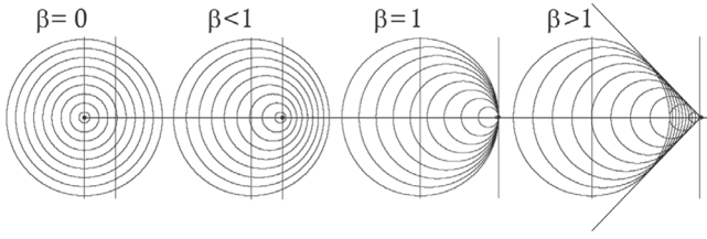
Fig. 2. Time reversal between sending and receiving for \beta = 1 , the sound barrier for the sound wave. For \beta > 1 , the most recently emitted wavefronts are received first.
