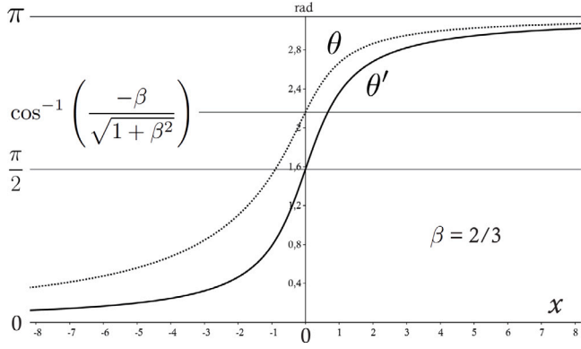
Fig. A.2. Plots of Galilean angular aberration as a function of distance. Dashed curve: Angle \theta between the trajectory of the source and the source–receiver direction according to Eq. (A.10). Solid line curve: angle \theta' between the trajectory of the source and the line connecting the emission point to the receiver.
