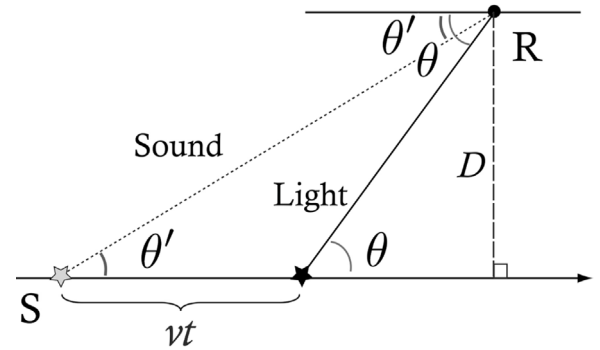
Fig. 7. Since the speed of light can be considered as infinite compared to that of sound, the sound wave carrying the Doppler effect emitted by the source S at an angle \theta' toward the receiver R , and the light carrying the image of the source, emitted at an angle \theta toward the receiver, arrive together at the receiver. D is the shortest distance between the source and the receiver on the entire trajectory.
