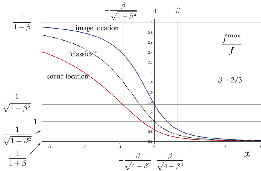
Fig. A.3. Doppler effect of the sound as a function of the relative position of a moving source on its path, for a stationary receiver in the absence of wind, expressed as a function of either the coordinate of the emitting point (lower red curve drawn to Eq. (A.7)), or of the visually detected source (upper blue curve drawn to Eq. (A.6)). The dashed black curve shown for comparison is that of the classical Doppler formula drawn to Eq. (A.5). The increment of the coordinate x is the minimum distance between the source and the receiver. (For interpretation of the references to color in this figure legend, the reader is referred to the web version of this article.)
