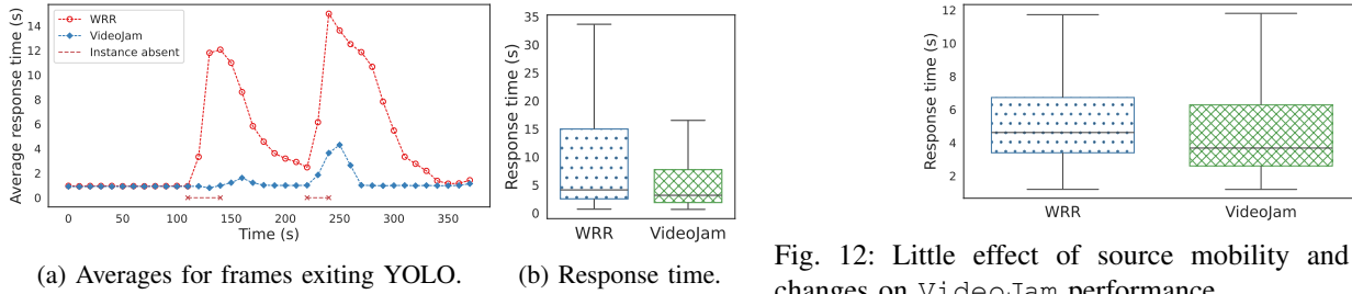
Fig. 11: Evaluation under node failure conditions: WRR's poor performance and VideoJam's adaptability under failures.
