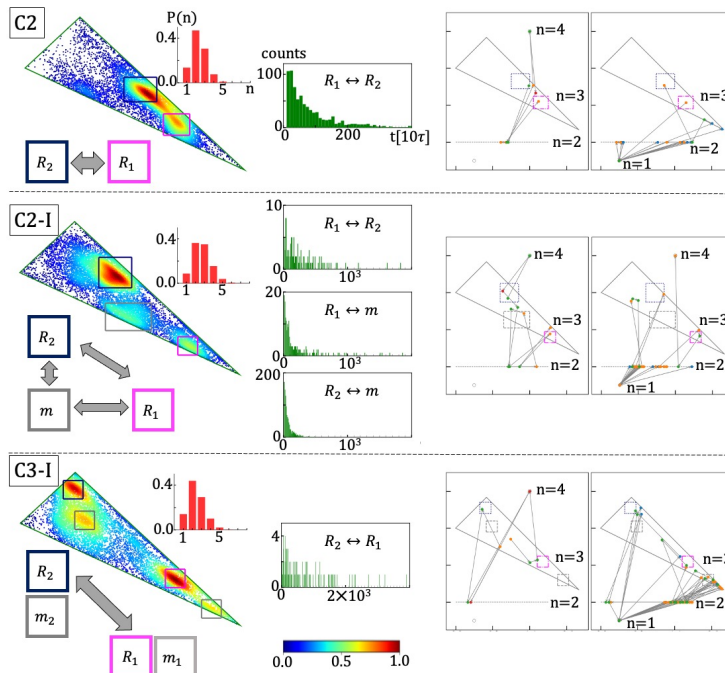
Figure 7: Trajectories of switching events between distant conformations in (a) C2 and in hybrids (b) C2-I and (c) C3-I. The left panels show the probability distribution P(n) of n -pearl states for the given sequence, along with a triangular diagram representing the density of visits. The middle panels show the distributions of switching times between marked regions in 2-simplexes for C2, C2-I and C3-I. The average switching times are 126\tau , 287\tau and 738\tau with rms deviations of 309\tau , 360\tau , 835\tau for C2, C2-I and C3-I, respectively. In C2-I, switching between R_1 and m , R_2 and m have average times of 242\tau and 97\tau . The right panels show typical short ( < 100\tau ) and long ( \sim 1000\tau ) trajectories on simplex representations. The trajectories start at the time leaving from one of the marked box ( R_2 ) and end at the time entering the marked magenta box ( R_1 ). 1-pearl state is a point, 2-pearl state as a 1-simplex x_1 \in [0, 0.5] , 3-pearl state is triangular 2-simplex \{x_1, x_2\} . The states with larger number of pearls ( n \geq 4 ) are shown as a point above the 2-simplex for convenience.
