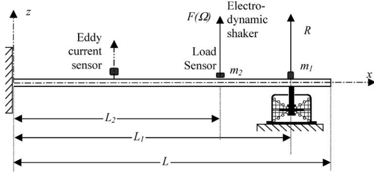
Fig. 7. Beam-isolator system in bending.
