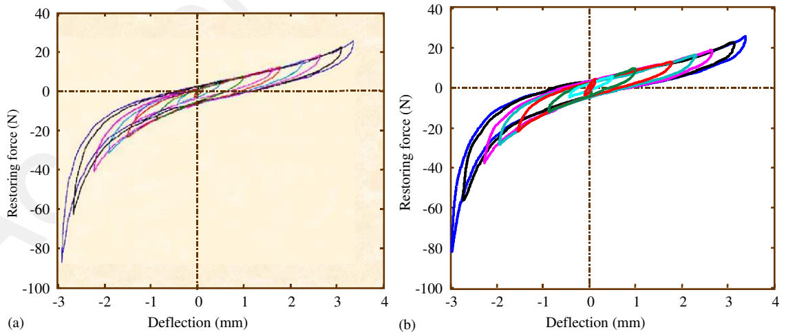
Fig. 3. Measured (a) and simulated (b) harmonic loops.
