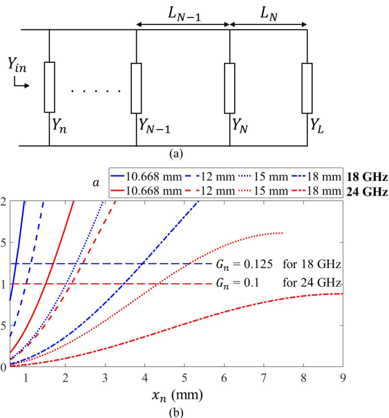
Fig. 2. (a) Equivalent circuit model of a longitudinal slot-loaded waveguide, (b) Normalized slot conductance G_n against slot offset x_n , at 18 GHz and 24 GHz considering different values of a
