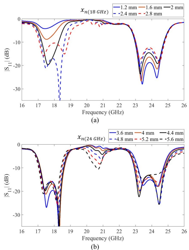
Fig. 5. Simulated |S_{11}| responses of the proposed antenna for different values of (a) x_n(18 \text{ GHz}) , and (b) x_n(24 \text{ GHz})
