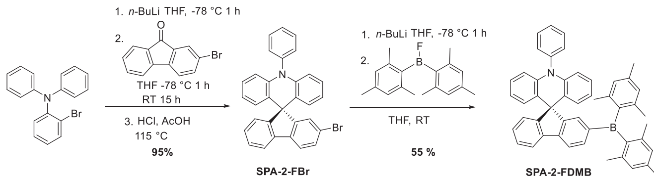
Scheme 1. Synthetic pathway of SPA-2-FDMB.
