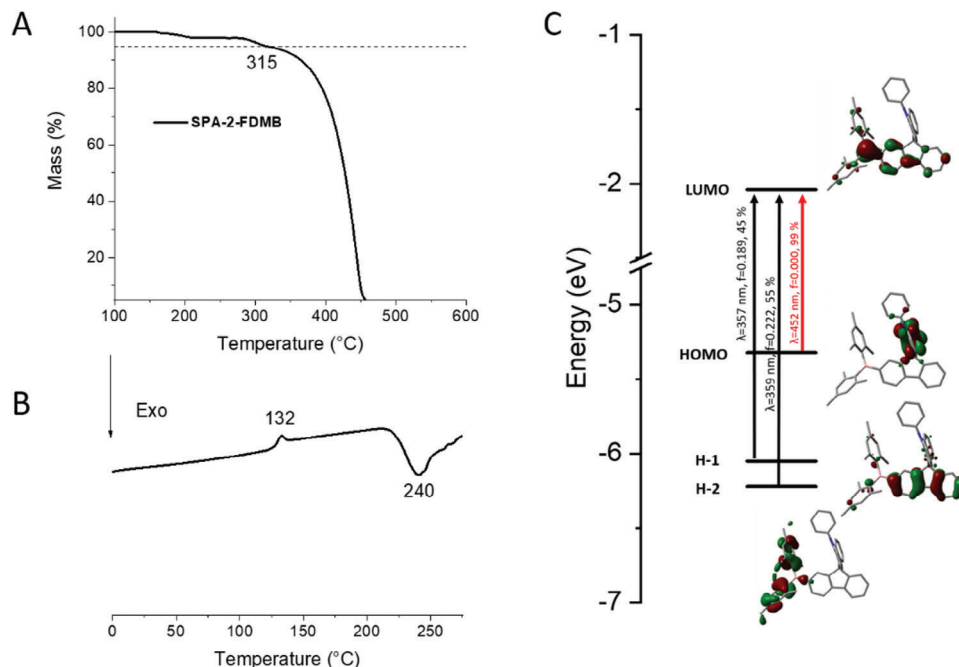
Figure 4. A) TGA and B) DSC (2 nd heating only) traces of SPA-2-FDMB, and C) representation of the energy levels and the main molecular orbitals involved in the electronic transitions obtained by TD-DFT, B3LYP/6–311+G(d,p), shown with an isovalue of 0.04 [ebohr -3 ] 1/2 . For clarity purposes, only the major contribution of each transition is shown (see Supporting Information for details).
