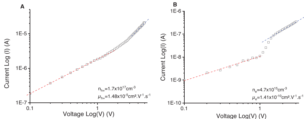
Figure 5. Thickness-scaled current-voltage characteristics of SPA-2-FDMB hole-A) and electron-only B) SCLC devices.
