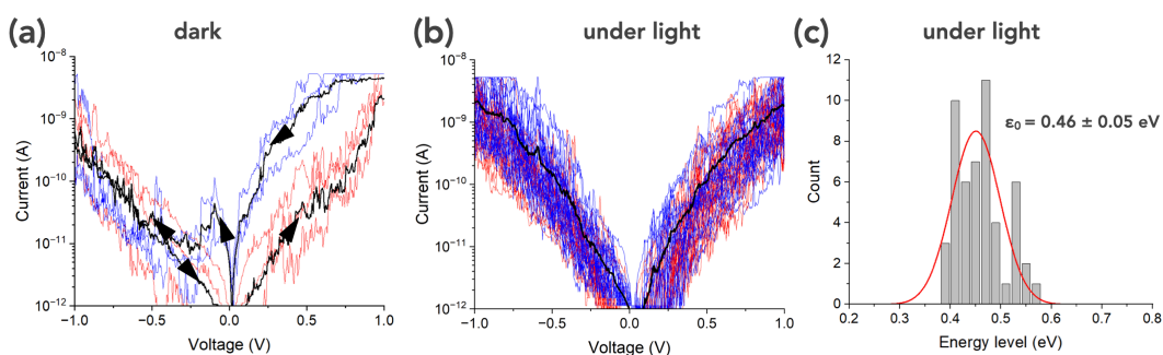
Figure 5. (a) Typical I-V curves in the dark of the TS Au-S-C 8/11 -Fc/AgNC/C-AFM tip junctions (other NCs than in Fig. 2). Only a few traces were recorded to check the hysteresis and NDC. The dark lines are the mean \bar{I} -V for the forward (red) and backward (blue) traces. (b) I-V data set (45 traces) of the TS Au-S-C 8/11 -Fc/AgNC/C-AFM tip junction under light illumination (470-850 nm wavelength). The back line is the mean \bar{I} -V from all the traces. (c) Histograms of energy level \epsilon_0 of the MOs involved in the ET under illumination (SEL model applied on data shown in Fig. 5b). The lines are the fit with Gaussian distributions with the values (mean \pm standard deviation) given in the panel.
