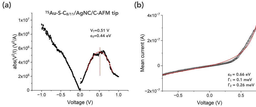
Figure S4. (a) Data of the mean \bar{I} - V of the ^{TS}\text{Au-S-C}_{8/11}/\text{AgNC/C-AFM} tip junction plotted as |V^2/I| vs. V . Only one maximum is detected. (b) Fit (red curve) of the SEL model (Eq. S4) on the mean \bar{I} - V of ^{TS}\text{Au-S-C}_{8/11}/\text{AgNC/C-AFM} tip junction fit limited between -0.75 and 0.75 V (vide supra), the fit parameters are given in the panel.
