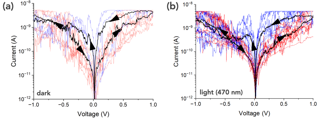
Figure S10. (a) Typical I - V curves in the dark of the ^{TS}\text{Au-S-C}_{8/11}\text{-Fc/AgNC/C-AFM} tip junctions (same sample but other NCs than in Fig. 5). Only a few traces (10) were recorded to check the hysteresis and NDC. The dark lines are the mean \bar{I} - V for the forward (red) and backward (blue) traces. (b) I - V data set (21 traces) of the ^{TS}\text{Au-S-C}_{8/11}\text{-Fc/AgNC/C-AFM} tip junction under light illumination at 470 nm (bandwidth : FWHM 20 nm). The dark lines are the mean \bar{I} - V for the forward (red) and backward (blue) traces.
