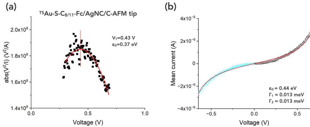
Figure S5. (a) Data of the mean \bar{I} - V of the ^{TS}\text{Au-S-C}_{8/11}\text{-Fc}/\text{AgNC/C-AFM} tip junction plotted as |V^2/I| vs. V . Only the backward trace from 1 to 0 V is used (see main text). (b) Fit (red curve) of the SEL model (Eq. S4) on the mean \bar{I} - V of ^{TS}\text{Au-S-C}_{8/11}/\text{AgNC/C-AFM} tip junction. Since an accurate fit of Eq. 1 requires to have data at positive and negative voltages (for the two arctan functions) a symmetric negative branch was added (light blue) by inverting the measured positive branch. The agreement is good with the TVS determination. The fit parameters are given in the panel.
