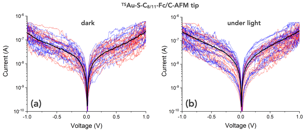
Figure S11. (a) I - V data set (40 traces) in the dark of the ^{TS}\text{Au-S-C}_{8/11}\text{-Fc/C-AFM} tip junctions. The dark line is the mean \bar{I} - V for all the traces. (b) I - V data set (40 traces) of the ^{TS}\text{Au-S-C}_{8/11}\text{-Fc/C-AFM} tip junction under light illumination (470-850 nm wavelength). The back line is the mean \bar{I} - V from all the traces.
