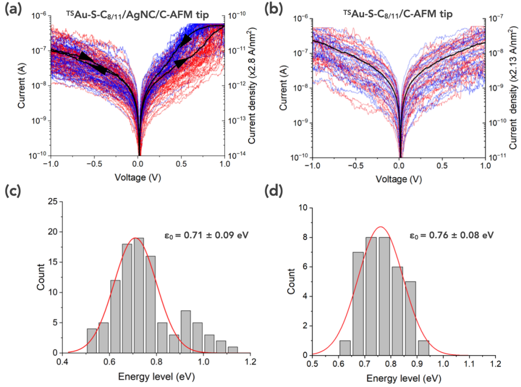
Figure 4. (a) I-V data set (120 traces) of the {}^{\text{TS}}\text{Au-S-C}_{8/11}/\text{AgNC}/\text{C-AFM} tip junction. The dark lines are the mean \bar{I} -V for the forward (red) and backward (blue) traces. (b) I-V data set (49 traces) of the {}^{\text{TS}}\text{Au-S-C}_{8/11}/\text{C-AFM} tip junction. The back line is the mean \bar{I} -V from all the traces. The current density scales are calculated with the estimated areas of the AgNC and C-AFM tip, respectively (see the Supporting Information). (c-d) Histograms of energy level \epsilon_0 of the MOs involved in the ET. The lines are the fit with Gaussian distributions with the values (mean \pm standard deviation) given in the panels: (c) {}^{\text{TS}}\text{Au-S-C}_{8/11}/\text{AgNC}/\text{C-AFM} tip junctions, from I-V datasets shown in Fig. 4a, (d) {}^{\text{TS}}\text{Au-S-C}_{8/11}/\text{C-AFM} tip junctions, from I-V datasets shown in Fig. 4b.
