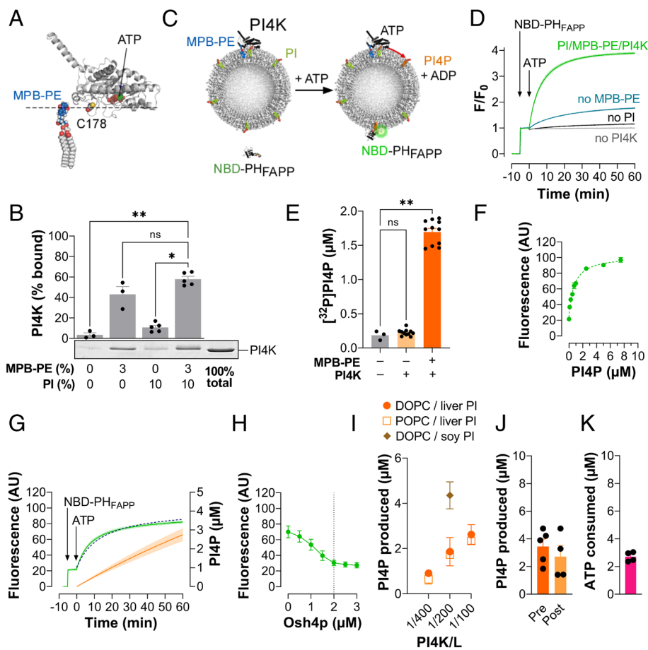
Fig. 1. PI4P synthesis on the liposome surface by membrane-associated PI 4-kinase. (A) Structure of PI4KII \alpha^{SSPS}\Delta C in complex with an ATP molecule (PDB ID: 4HNE; ATP is represented in sphere mode, with carbon in green, nitrogen in blue, oxygen in red, and phosphorus in orange). A serine residue (S178) in the SSPS sequence was replaced by a cysteine residue (represented in sphere mode, carbon in gray, sulfur in yellow). The orientation of the kinase relative to the membrane surface (dashed line) was suggested by molecular dynamics simulations (40). A molecule of MPB-PE is represented with carbon in gray (glycerol and acyl chain) or dark blue (headgroup), oxygen in red, nitrogen in blue, phosphorus in orange, and hydrogen in white. The figure was prepared using PyMOL ( http://pymol.org ). (B) Flotation assays. PI4K (4 \mu\text{M} ) was mixed with liposomes (800 \mu\text{M} lipids) only made of DOPC or containing 10% liver PI, 3% MPB-PE, or both lipids in HK buffer at 25 ^{\circ}\text{C} for 1 h. The functionalization reaction was stopped by adding 1 mM DTT. After centrifugation, the liposomes were recovered at the top of sucrose cushions and analyzed by sodium dodecyl-sulfate polyacrylamide gel electrophoresis (SDS-PAGE). The amount of membrane-bound PI4K was determined using the content of lane 5 (100% total) as a reference based on the SYPRO Orange signal. Data are represented as mean \pm SEM ( n = 3 to 5) with single data points. Kruskal-Wallis with Dunn's multiple comparison test ( *P < 0.05 and **P < 0.01 ). (C) Principle of PI4P detection in the membrane coated with PI4K using NBD-PH _{FAPP} . ATP is added to PI-containing liposomes functionalized with PI4K. If PI4P is synthesized, NBD-PH _{FAPP} binds to the liposomes and becomes more fluorescent. (D) Liposomes (800 \mu\text{M} ) composed of DOPC/liver PI/MPB-PE (87/10/3) were mixed for 1 h with 4 \mu\text{M} of DTT-free PI4K (PI4K/L molar ratio = 1/100 considering only lipids in the outer leaflet). This mixture was diluted fourfold in 600 \mu\text{L} HK buffer containing 7 mM MgCl _2 (HKM7 buffer). Then, NBD-PH _{FAPP} (250 nM) and ATP (100 \mu\text{M} ) were sequentially injected. Control experiments were conducted without PI4K or with liposomes devoid of MPB-PE or PI. The signal was measured at \lambda = 525 nm ( \lambda_{ex} = 495 nm). The fluorescence was normalized to the F_0 fluorescence recorded before the last injection. Each trace is the mean \pm SEM of kinetics recorded in independent assays (green trace, PI-containing liposomes coated with PI4K, n = 4 ; blue-green trace, liposomes without MPB-PE, n = 3 ; black trace, PI-free liposomes, n = 3 ; gray trace, without PI4K, n = 4 ). (E) Kinase assay. [ \gamma - ^{32}\text{P} ]ATP (100 \mu\text{M} ) was added to DOPC liposomes (200 \mu\text{M} ) containing 10% PI, with or without 3% MPB-PE, and preincubated for 1 h with PI4K (PI4K/L = 1/200). Control experiments were conducted with PI-containing liposomes alone. The reaction was allowed to proceed for 1 h at 30 ^{\circ}\text{C} under agitation. The lipids were extracted and dried. The radioactivity in the reaction mix and associated with lipids was counted to quantify newly made PI4P. Orange bars, with MPB-PE-containing liposomes; light-orange bars, with MPB-PE-free liposomes; gray bars, without PI4K. Data are represented as mean \pm SEM ( n = 3 to 11). Kruskal-Wallis with Dunn's multiple comparison test; **P < 0.01 , ns: P \geq 0.05 . (F) Fluorescence of NBD-PH _{FAPP} (250 nM) incubated with liposomes (200 \mu\text{M} ) made of DOPC and containing increasing amounts of PI4P at the expense of PI [with PI + PI4P accounting for 10% of lipids]. The intensity F is given as a function of the volume concentration of PI4P, resulting in a binding curve that can be fitted considering F = F_0 + F_b \times [\text{PI4P}]/([\text{PI4P}] + K_d) and a 1:1 stoichiometry. (G) Determination of PI4P production. Liposomes (800 \mu\text{M} ), composed of DOPC/liver PI/MPB-PE (87/10/3) and functionalized with PI4K (PI4K/L = 1/100), were diluted fourfold in HKM7 buffer. Then, NBD-PH _{FAPP} (250 nM) and ATP were added. The fluorescence signal was measured at 525 nm ( \lambda_{ex} = 495 nm, green trace) and corrected for photobleaching. The data points were fitted (dotted curve, considering a pseudo-first-order reaction) to determine the rate of PI4P synthesis and calculate the amount of PI4P produced over time (orange curve, SI Appendix ). Mean \pm SEM ( n = 3 to 4). (H) Incremental amounts of Osh4p were added to liposomes at the end of kinetics shown in (G). A minimal signal was reached once 2.5 to 3 \mu\text{M} Osh4p was added (dashed lines), suggesting that a similar amount of PI4P was present in the outer leaflet of liposomes and extracted by the protein. (I) Amount of PI4P synthesized after 1 h in DOPC or POPC membranes enriched with 10% liver PI (mostly 18:0/20:4-PI) or soy PI (mostly 16:0/18:2-PI) and functionalized with a variable quantity of PI4K. Mean \pm SEM ( n = 3 to 5). (J) Amount of PI4P produced in PI-containing membranes functionalized with PI4K within 1 h following ATP addition estimated by fitting the kinetics traces shown in SI Appendix , Fig. S3C (orange bars, nonisolated liposomes; light-orange bars, isolated liposomes). Mean \pm SEM ( n = 4 to 5). (K) Amount of ATP hydrolyzed in 1 h by PI4K at the surface of PI-containing liposomes used for assays shown in SI Appendix , Fig. S3C. Mean \pm SEM ( n = 4 ).
