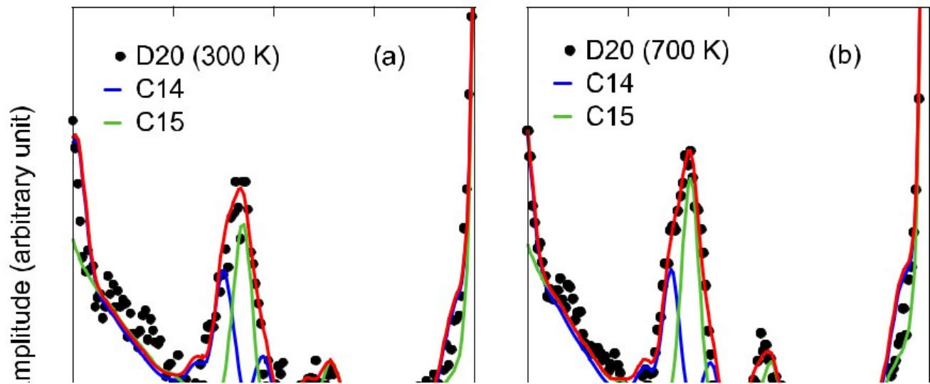
Fig. 12 Examples of Bragg peaks measured with D20 at 300 and 700 K corresponding to Zr(Fe,Cr)_2 (structures C14 and C15) and ZrO_2 (monoclinic and tetragonal phases). The red line represents the total contribution
