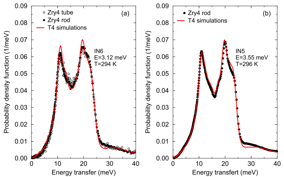
Fig. 8 Neutron-weighted multiphonon spectra measured at room temperature and simulated with TRIPOLI-4®
