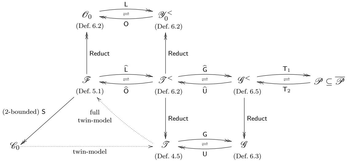
Figure 2: Relations between the classes of structures involved in the proof of the main result. The interpretation \mathbf{S} is defined in Definition 5.1, the transduction pairing (\mathbf{L}, \mathbf{O}) in Lemma 6.1, the transduction pairing (\widehat{\mathbf{L}}, \widehat{\mathbf{O}}) as a remark just after Definition 6.2, the transduction pairing (\widehat{\mathbf{G}}, \widehat{\mathbf{U}}) in Lemma 6.4, and the transduction pairing (\widehat{\mathbf{G}}, \widehat{\mathbf{U}}) as a remark just after Definition 6.5.
