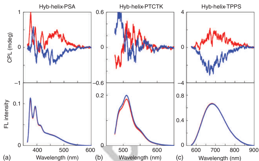
Figure 8.10 CPL and fluorescence spectra of (a) PSA (ex 340 nm), (b) PTCTK (ex 430 nm), and (c) TPPS (ex 410 nm) in the presence of RH- (red line) or LH- (blue line) handed hybrid helices. Source: Reproduced with permission from Scalabre et al. [44]/John Wiley & Sons.
