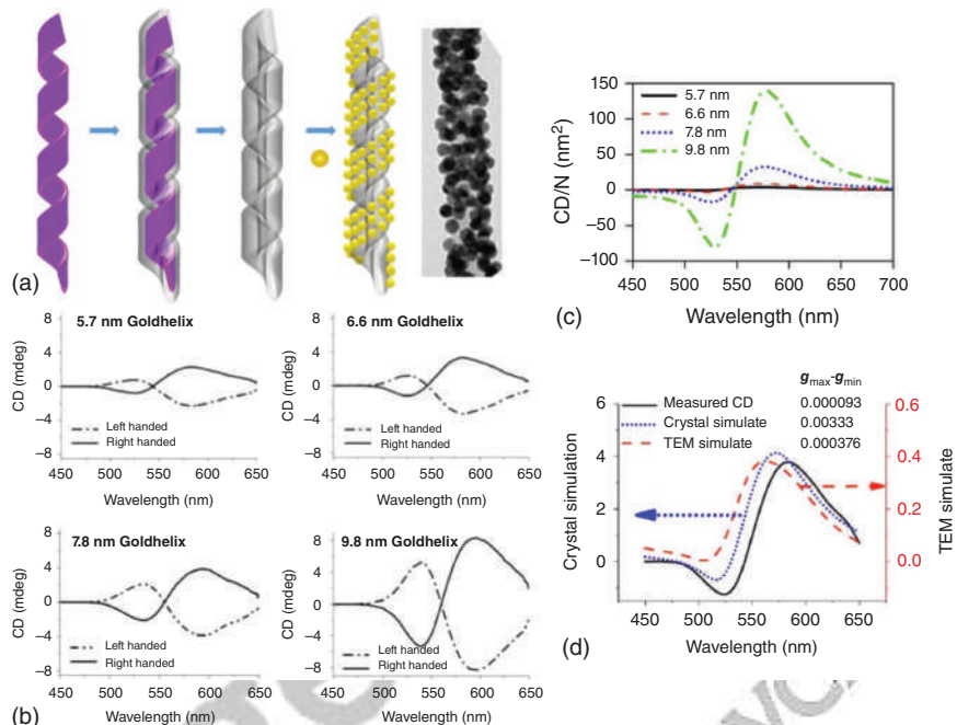
Figure 8.5 Silica nanohelices synthesized from sol-gel condensation of TEOS on self-assembled organic nanostructures are used as a matrix to prepare helical GNPs superstructures (Gold helix) with tunable and well-defined handedness. (a) Scheme of fabrication of GNPs@ SiO 2 helix. (b) Corresponding electronic CD spectra of the Gold helices for four different diameters. Dashed lines represent left-handed Gold helix, and solid lines represent right-handed Gold helix. (c) Influence of the GNP radius on the CD/N spectra simulated by considering perfectly aligned (crystalline organization) and monodisperse GNPs forming right-handed helical organization. (d) Measured CD signal obtained for 5.7 nm GNPs (black solid line) is compared with the simulated CD signal obtained for perfect crystalline organization ( \sigma = 0 , blue dotted line) as well as the CD signal simulated for the real position of the GNPs (3D tomography, red dashed line). Source: Reproduced with permission from American Chemical Society, 2018.
