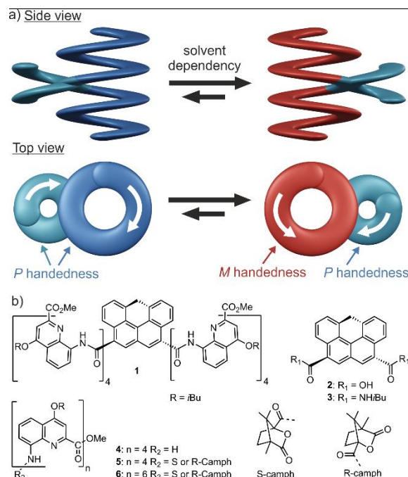
Fig. 1 a) Cartoon representation of the dual helicity in the fused helicene-foldamer architecture and the equilibrium between the PP and PM diastereoisomers. Note that the small diameter helix has a fixed handedness whereas the large diameter helix handedness is dynamic. Left ( M ) and right ( P ) handedness are colored in red and blue, respectively. b) Molecular formulas of the fused helicene/foldamer, the [4]carbohelicenes and the quinoline oligomers.
