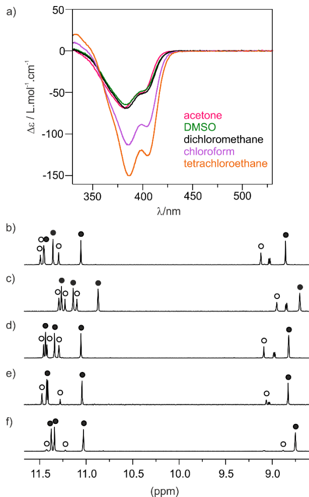
Fig. 3 a) ECD spectra of P - 1 (150 μM) recorded in DMSO (green), acetone (pink), dichloromethane (black), chloroform (purple) and tetrachloroethane (orange) at 298 K. Parts of the 1 H NMR spectra (700MHz) showing the amide signals of P - 1 (1.0mM) at 298K in b) acetone- d 6 ; c) DMSO- d 6 ; d) dichloromethane- d 2 ; e) chloroform- d ; and f) tetrachloroethane- d 2 . The amide signals of the major diastereoisomer are denoted with full black circles (●), while those of the minor species are marked with black circles (○).
