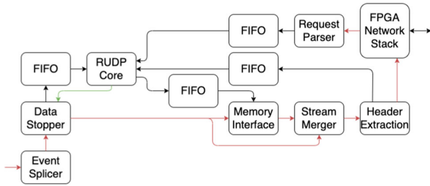
Fig. 18 Selective repeat protocol block diagram. Figure taken from Ref. [27]
