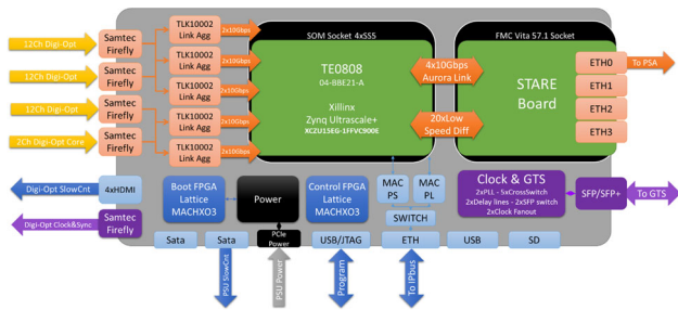
Fig. 8 The PACE pre-processing board block diagram
