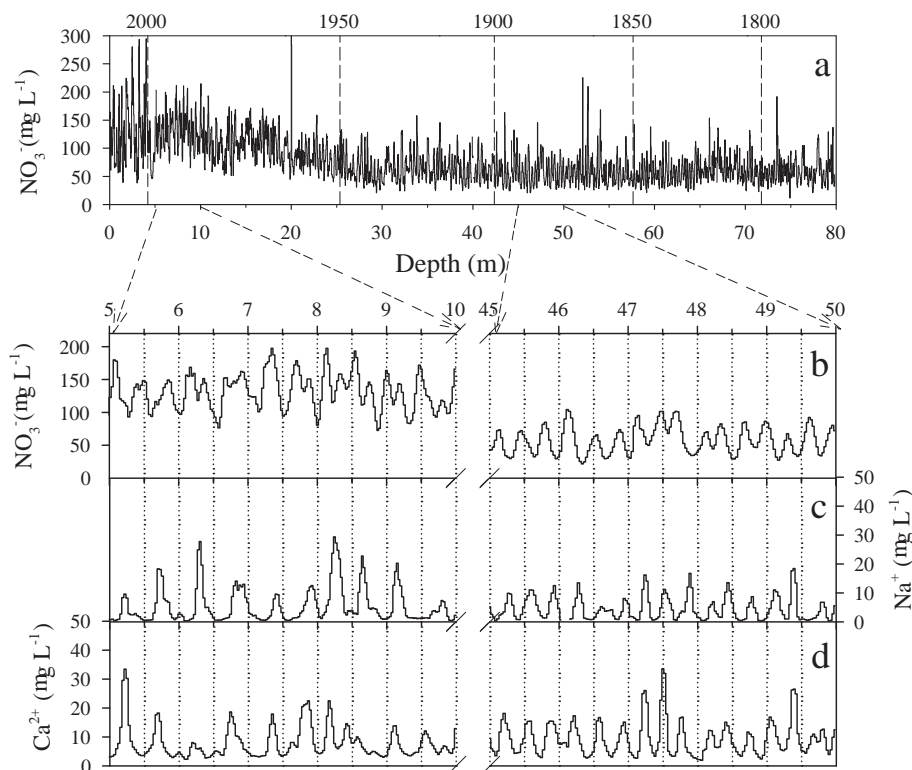
Figure 2. (a) Nitrate concentration record from the shallow ice core; (b–d) show seasonal peaks of \text{NO}_3^- , \text{Na}^+ and \text{Ca}^{2+} , respectively, in two sections of the ice core (data shown in b, c and d are 3-point running averages). Vertical dashed lines in (a) indicate the years of snowfall at relevant depths.
