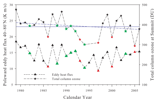
Figure 3. Summit springtime O 3 column density (February and March averages) and poleward eddy heat flux in the lower stratosphere (40–80° N, January and February averages) from 1979 to 2006. The solid blue line is the average of springtime O 3 column density from 1979 to 2006 ( 390 \pm 50 ( 1\sigma ) DU), and the dashed blue line is the linear least-squared regression of the O 3 column density from 1979 to 2006. The symbols marked as red and green indicate years with double nitrate peaks, while the green symbols indicate one of the double nitrate peaks is accompanied with a sulfate peak.
