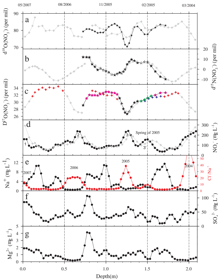
Figure 1. \delta^{18}\text{O}(\text{NO}_3^-) (a), \delta^{15}\text{N}(\text{NO}_3^-) (b), \Delta^{17}\text{O}(\text{NO}_3^-) (c) and concentrations of \text{NO}_3^- (d), \text{Na}^+ (e), \text{SO}_4^{2-} (f) and \text{Mg}^{2+} (g) in the snow samples (data are 3-point running averages). SP-1 data were plotted in gray with plus signs; SP-2 and SB data were plotted in black with circle and star signs, respectively. The pink and green stars represent samples in SB used to calculate the winter and 2005 spring mean \Delta^{17}\text{O}(\text{NO}_3^-) , respectively; the red and blue plus signs represent samples in SP-1 used to calculate the winter and 2005 spring mean \Delta^{17}\text{O}(\text{NO}_3^-) , respectively. The vertical dashed line indicates the approximate months of snowfall at depths of 0, 0.5, 1.0, 1.5 and 2.0 m by method B as described in the text.
