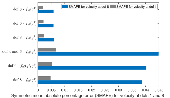
Fig. 7. SMAPE values of the state estimation with rKF for different functional forms and location of nonlinearities. Velocities at dof 1 and dof 8.
