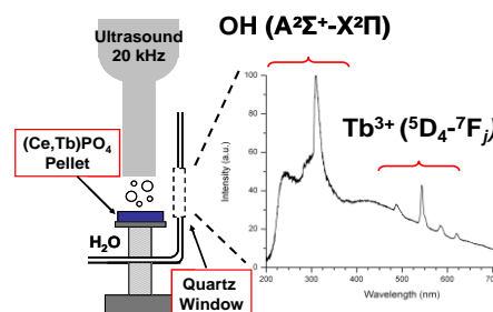
Fig. 1 : SL spectra observed during the sonication of (\text{Ce}_{0.9}\text{Tb}_{0.1})\text{PO}_4 pellet
