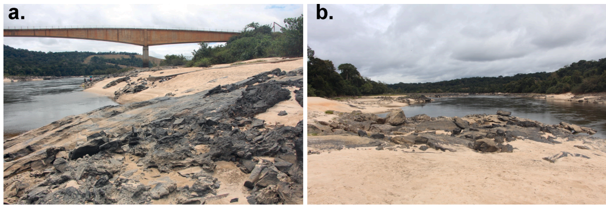
Fig. 2. Photos of the sampling sites along the Ogooué River at Ayem (sampling site #26), upstream (note the people for scale) and downstream. Sand was sampled from the banks at this site.
