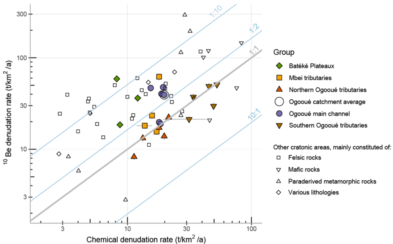
Fig. 11. Millennial ^{10}\text{Be} -derived denudation rates vs. modern solute specific flux (in logarithmic scale) for ORB and other rivers draining cratonic areas worldwide: Oubangi, Congo, Niger, Zambesi, Fish, Molopo, Orange, Okavango, Limpopo, Murray and Darling, Finke, Macumba, Neales, St. Lawrence, Mississippi, Volga, Dniepr, Lena (Wittmann et al., 2020); Mpanga North, Dunga, Igasa, Ruimi, Mobuku, Isebo, Kilembe, Mpanga South, Dura (Hinderer et al., 2013); Maracuja, Caraca (Salgado et al., 2007); Cristiano Otoni, Sao Geraldo (Cherem et al., 2012b, 2012a); Selenga, Turka, Barguzin, Upper Angara, Kichera (Suhroff et al., 2022); Nyong, Mengong, Bivesse, Awout, Soo, Mbam, Sanaga (Regard et al., 2016), Branco and Tapajos (Filizola and Guyot, 2009; Wittmann et al., 2011). The lithology indicated in the legend has been evaluated from the original publications and from the GLiM database (Hartmann and Moosdorf, 2012). The lines show the particular ratios between the chemical denudation and ^{10}\text{Be} denudation rates; the 1:1 line depicts the equivalent denudation rates. [Printed in Black & White]. (For interpretation of the references to color in this figure legend, the reader is referred to the web version of this article.)
