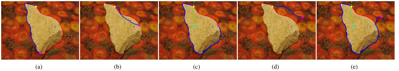
Fig. 4. Examples of minimal paths associated to asymmetric quadratic metric for boundary detection. The yellow and magenta dots are respectively the source points and endpoints of the minimal paths. a Two minimal paths form a simple closed contour, since their source points and endpoints are distributed evenly at the target boundary. b and d Minimal paths associated to source points and endpoints which are close to each other, where the blue lines suffer from a shortcut problem. c and e Minimal Paths in conjunction with adaptive cuts (green dash lines), where the yellow dots are the source points \mathbf{s} lying in the adaptive cuts.
