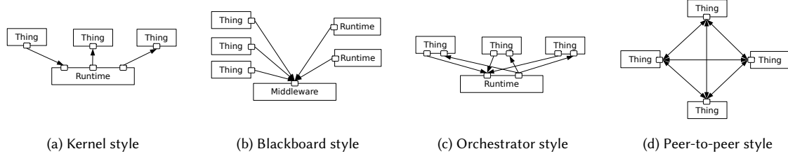
Fig. 3. Common architectural styles for IoT platforms ( \square : component, \square : connector, \rightarrow : connection)
