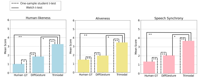
Figure 4: Statistical comparison of mean scores for each model and each aspect (Human-likeness, Aliveness, and Speech synchrony). The lines represent a significant superiority between the two values. Dotted lines correspond to Student t-tests and plain lines to Welch t-tests. * means p-value < 0.05 while ** means p-value < 0.01
