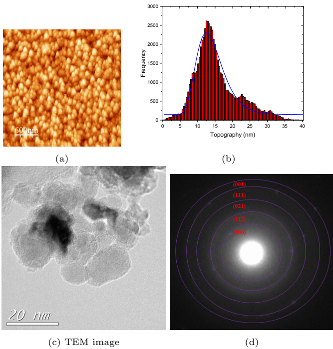
Figure 2: (a) AFM image and its corresponding (b) particle size distribution after 60 min of deposition on a silicon substrate. (c) TEM image and (d) its corresponding selected area electron diffraction of carbon nanoparticles deposit for 5 min of deposition in the cold finger. Experimental conditions: \text{CH}_4 = 4 sccm, \text{H}_2 = 96 sccm, reactor pressure = 100 mbar, absorbed power = 90 W )
