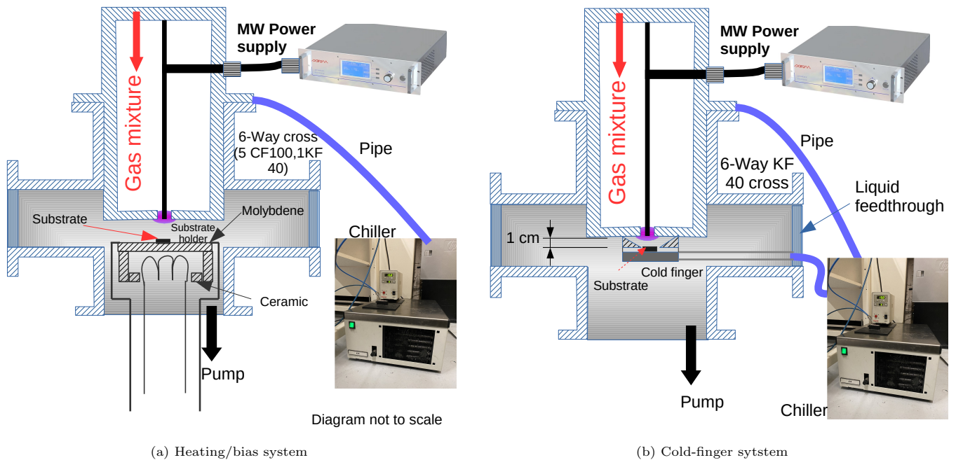
Figure 1: Experimental set-up for carbon particle deposition using the MW microplasma torch
