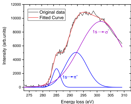
(a) EELS spectra of carbon nanoparticles deposit for 5 min of deposition in the cold finger
