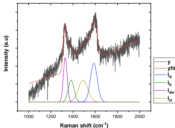
(b) Raman spectrum deconvolution
