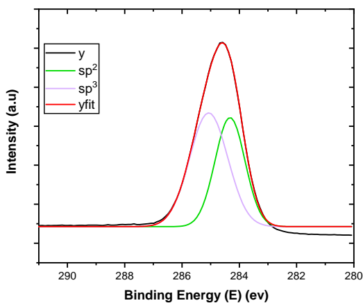
(c) Deconvolution of XPS C1s line to sp^3/sp^2 configuration
