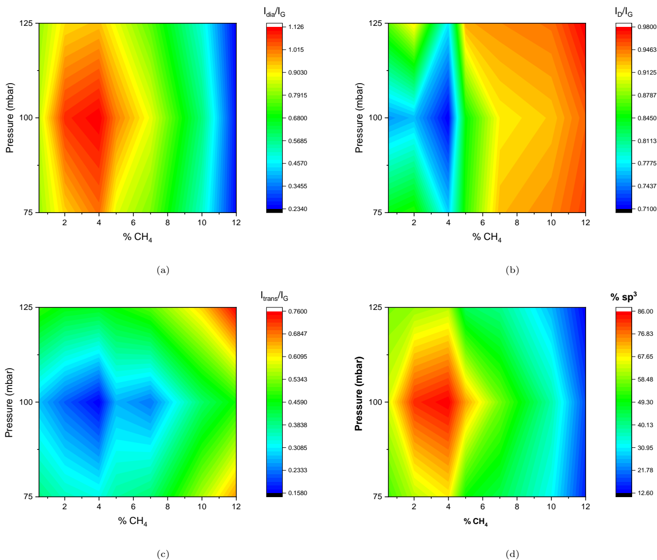
Figure 4: Distribution of (a) I_{dia}/I_G , (b) I_D/I_G , (c) I_{trans}/I_G and (d) %sp 3 as a function of pressure and methane concentration. Experimental conditions: Pressure = 100 mbar, injected power = 90 W, substrate = silicon, distance plasma-substrate = 1cm and deposition time = 1h.
