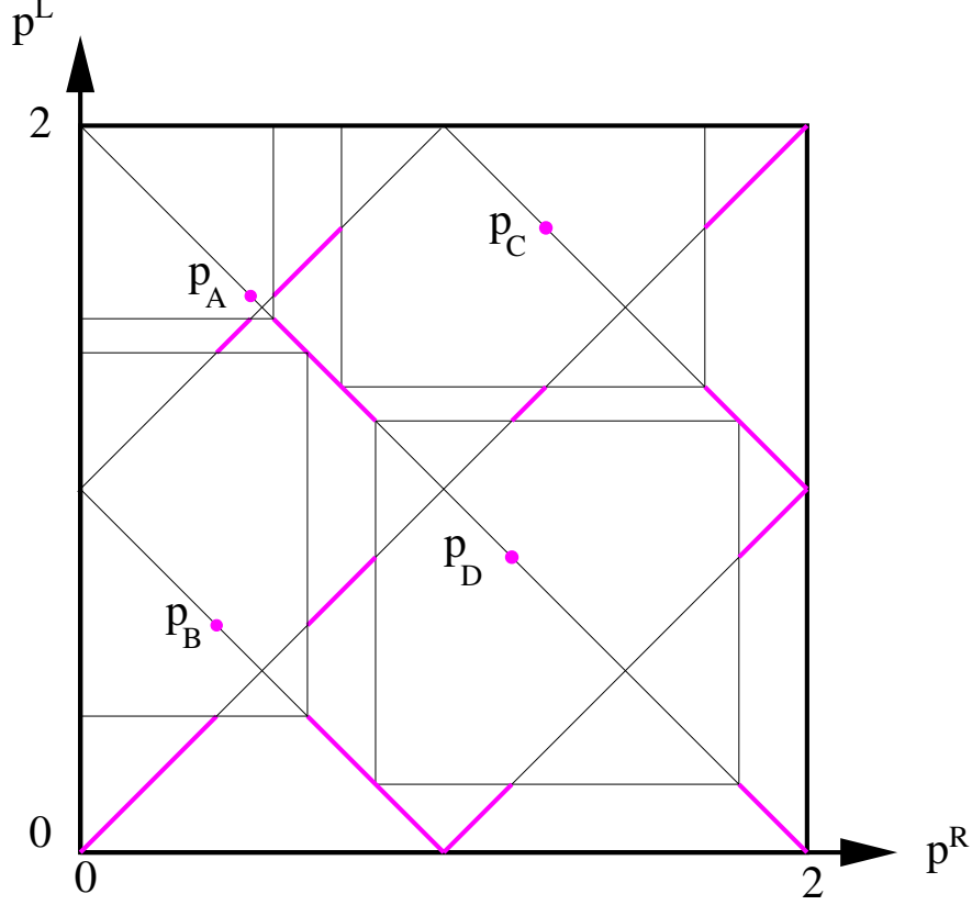
Figure 4: HJ Germ \mathcal{G}_A \subset \{g(p^L) = g(p^R)\} and characteristic subset \chi\mathcal{G}_A = \{p_A, p_B, p_C, p_D\}
