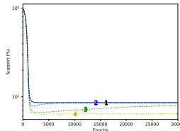
Fig. 3. rcv1_train dataset
