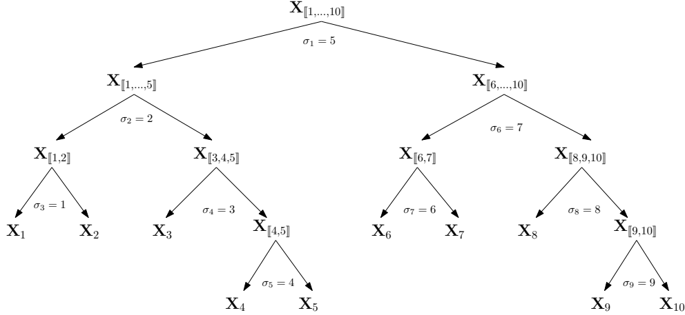
Fig. 7: Illustration of the permutation \sigma = (5, 2, 1, 3, 4, 7, 6, 8, 9) corresponding to the balanced factor-bracketing tree of \llbracket 10 \rrbracket .
