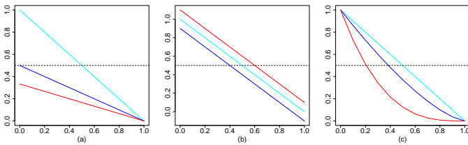
Figure 2: Representation of s : u \mapsto \delta(r - u)^{1/t} as a proxy of the parametric form of \sigma given in (2), with varying parameters. By default, all parameters are fixed to 1. We vary in (a) \delta \in \{1, 0.5, 1/3\} , in (b) r \in \{0.9, 1, 1.1\} , in (c) t \in \{1, 0.7, 1/3\} . The dashed line represents a constant threshold function \sigma = 0.5 .
