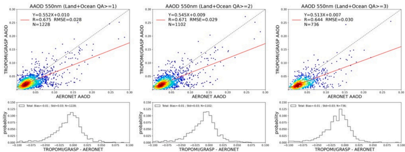
Fig. 12. Validation of TROPOMI/GRASP AAOD(550) with AERONET for an entire year (March 2019 to February 2020). From left to right: QA \geq 1, QA \geq 2 and QA \geq 3.
