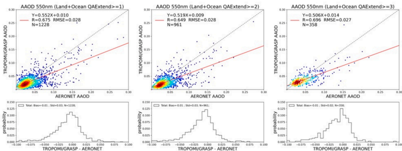
Fig. 13. The same as in Fig. 12 but for QAExtend index values.
