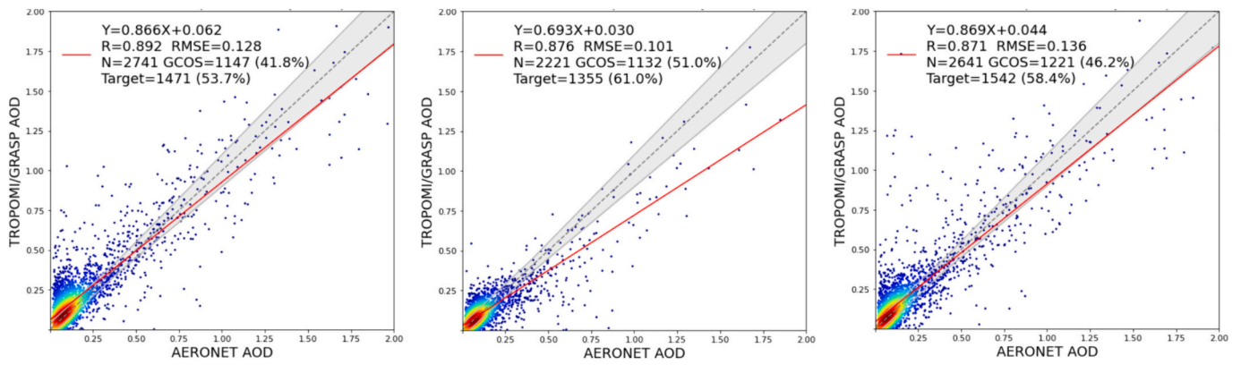
Fig. 1. TROPOMI/GRASP retrieval of aerosol properties over land vs AERONET. Left panel: the retrieval without using a priori estimates constraints (test (i)). Middle panel: initial guess from KNMI DLER TROPOMI climatology is used (test (ii)). Right panel: the results obtained when a_{vol} and a_{geom} BRDF parameters are constrained by the a priori estimates from POLDER/GRASP BRDF climatology (test (iii)).
