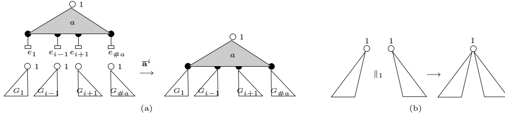
Figure 4: Tree operations: substitution (a) parallel composition (b)
