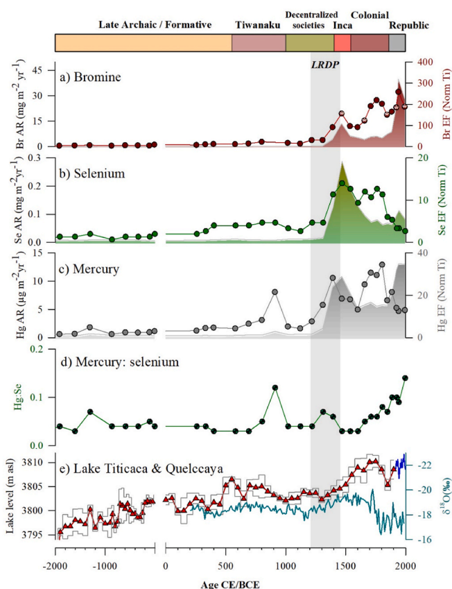
Fig. 6. Reconstruction of paleo-climate trace element proxies in Saitoco and comparison with published reconstructions of precipitations in the Altiplano. Panels a), b) and c) show the accumulation rates (AR) and enrichment factors (EF) of respectively bromine (Br), selenium (Se) and mercury (Hg). Samples used for XAS spectroscopy are indicated with a white star within dots in panel a). Panel d) gives the Hg:Se ratio, which reflects the anthropogenic Hg contribution when the ratio increases above the baseline ratio. Panel e) informs on variations in Lake Titicaca water level (red symbols; Guédron et al., 2023) and \delta^{18}O record (cyan line) of Quelccaya Ice core (Thompson et al., 2013) during the same time period. The vertical shaded grey highlights the Late Regional Development Period (LRDP).
