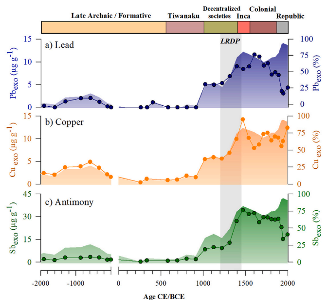
Fig. 8. Calculated exogenic concentrations (circles) and percentage of the total elemental concentration (areas filled) for a) lead (Pb), b) copper (Cu), and c) antimony (Sb).
