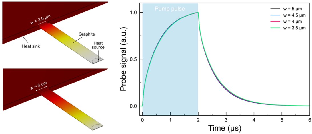
Extended Data Fig. 8 | Investigation of the effect of contact size on thermal conduction. FEM simulations in graphite ribbon with different contact areas at the heat sinks.
