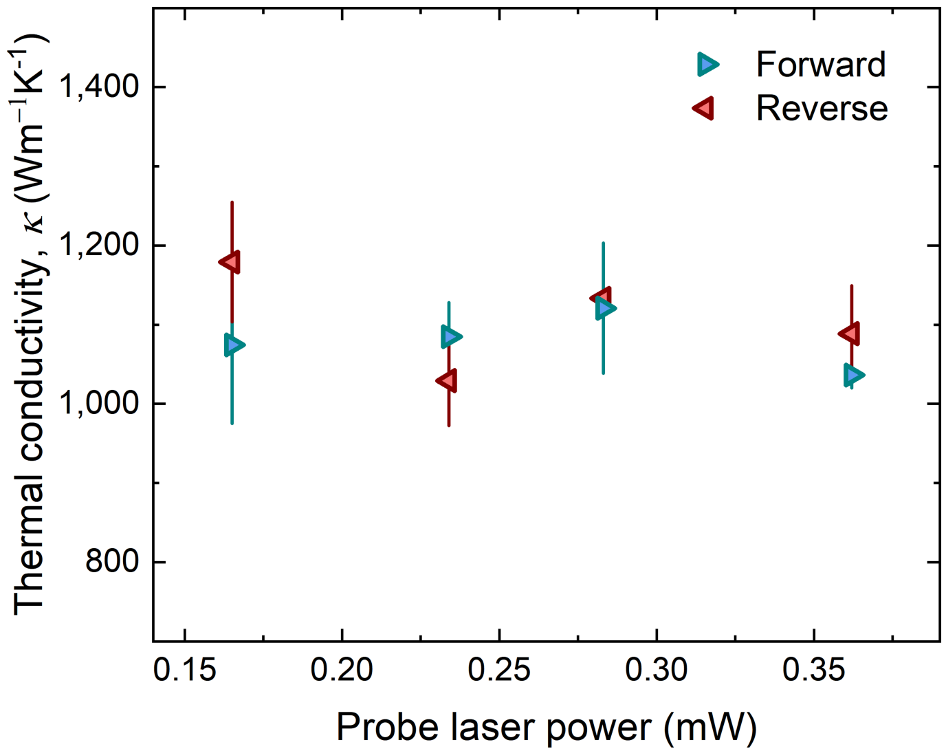
Extended Data Fig. 9 | Investigation of the laser heating effect in the \mu -TDTR system. Measured thermal conductivity of the graphite Tesla valve in the forward and reverse directions as a function of probe laser power in the \mu -TDTR system at 300 K.
