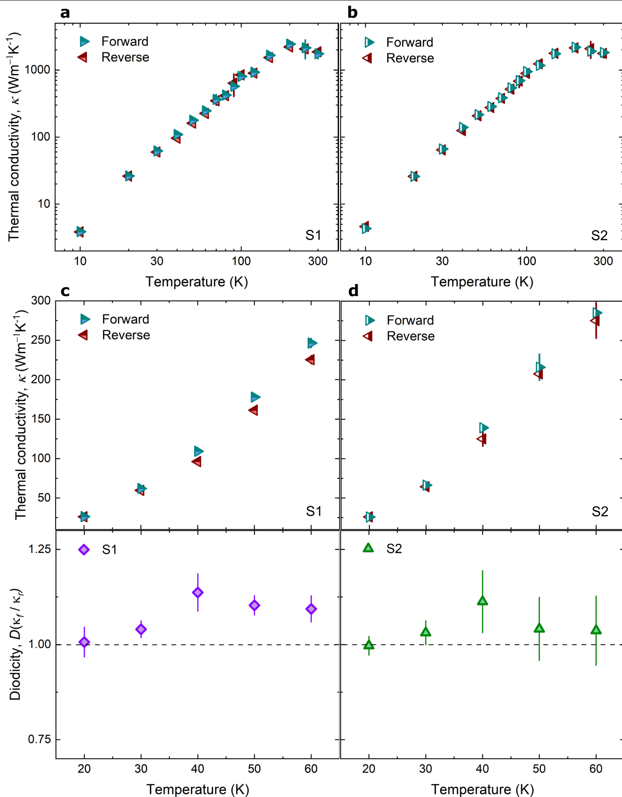
Extended Data Fig. 5 | Thermal rectification in the supplementary graphite Tesla valve sample within the hydrodynamic temperature range. Temperature-dependent thermal conductivity and diodicity of graphite Tesla
