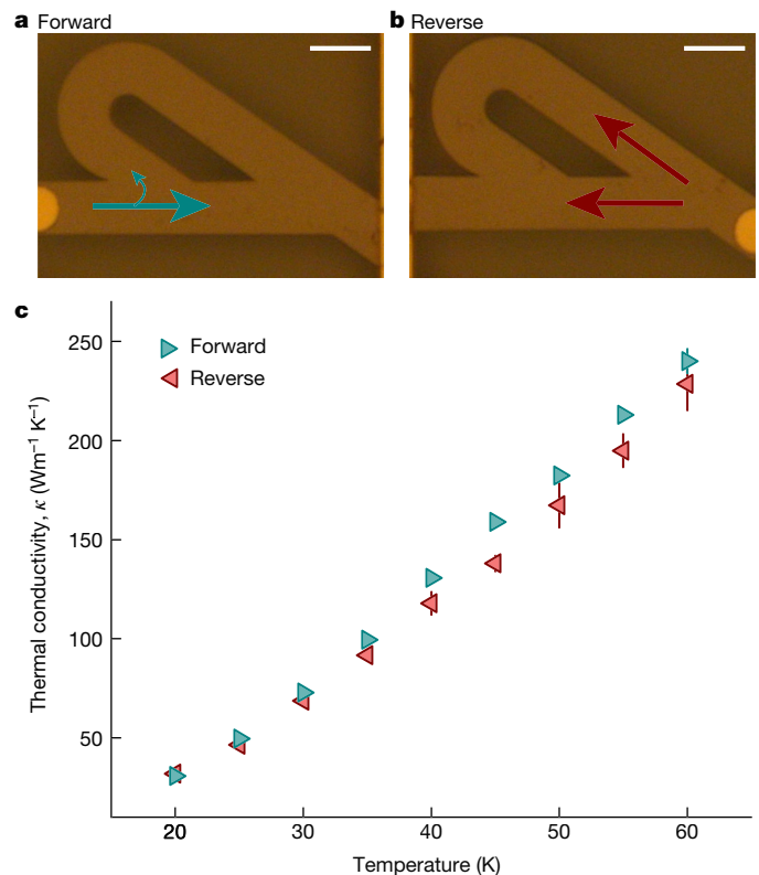
Fig. 3 | Thermal conductivity of the graphite Tesla valve. a, b , Optical microscope images of the graphite Tesla valve in forward and reverse directions, respectively. Arrows indicate the directions of heat flows. Scale bars, 5 \mu m. c , Thermal conductivity of the graphite Tesla valve in forward (cyan triangles) and reverse (red triangles) directions. Error bars denote the standard deviations ( \sigma ) of \kappa values from 3 to 10 measurements for each structure (forward or reverse) at a given temperature.
