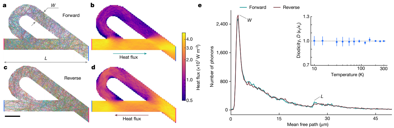
Fig. 2 | Monte Carlo simulations of the phonon Tesla valve. a–d , Phonon paths and heat-flux maps of the Tesla valve in forward ( a,b ) and reverse ( c,d ) directions at 10 K. Scale bar, 5 \mu m. e , Phonon mean-free-path spectra of the
