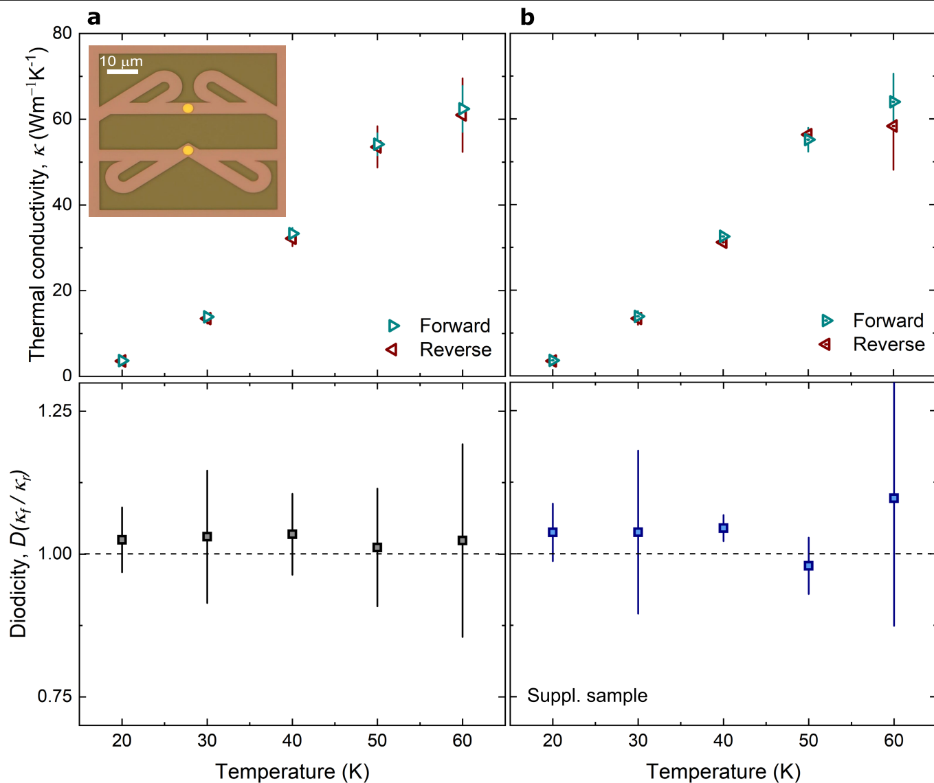
Extended Data Fig. 7 | Silicon Tesla valve within the hydrodynamic temperature range. a , Thermal conductivity and diodicity as a function of temperature from 20 to 60 K (hydrodynamic temperature range of graphite) in normal scale. Inset, optical microscope image of Tesla valves in the forward
