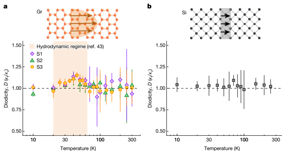
Fig. 4 | Thermal rectification in the graphite Tesla valve. a, b , Thermal diodicity (the ratio of thermal conductivity in the forward, \kappa_f , and reverse, \kappa_r , directions) as a function of temperature in graphite Tesla valve samples S1–S3 ( a ) and the silicon Tesla valve ( b ). The orange region shows the calculated phonon hydrodynamic temperature window of a 4.5- \mu\text{m} -wide graphite channel in our
