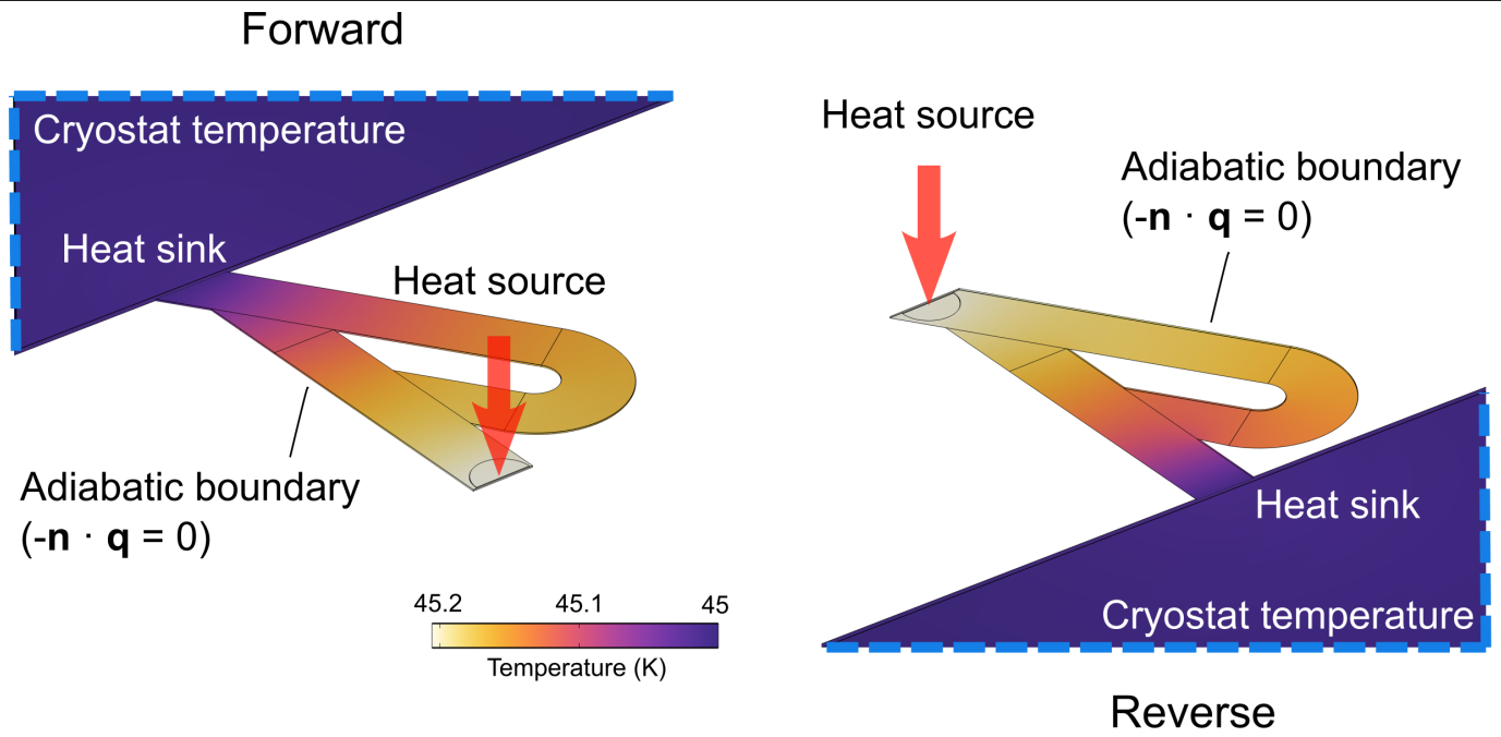
Extended Data Fig. 10 | FEM simulation model of the graphite Tesla valve. Illustration of heat dissipation in the graphite Tesla valve in both the forward (left) and reverse (right) directions in FEM models.
