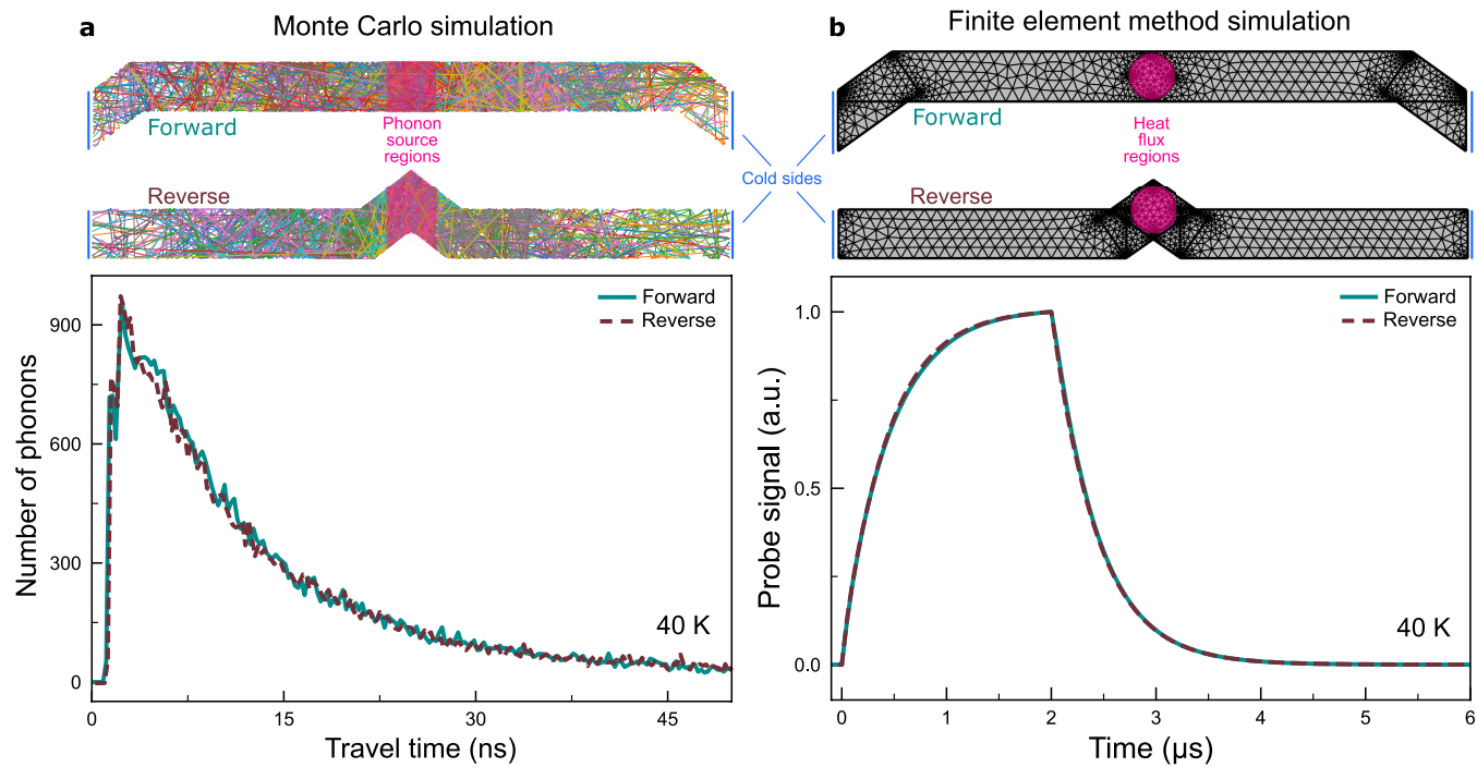
Extended Data Fig. 3 | Investigation of the effect of terminal geometry in the graphite Tesla valve. Monte Carlo (a) and FEM (b) simulations in the main channels of the Tesla valve with geometry difference at the sources and the sinks.
