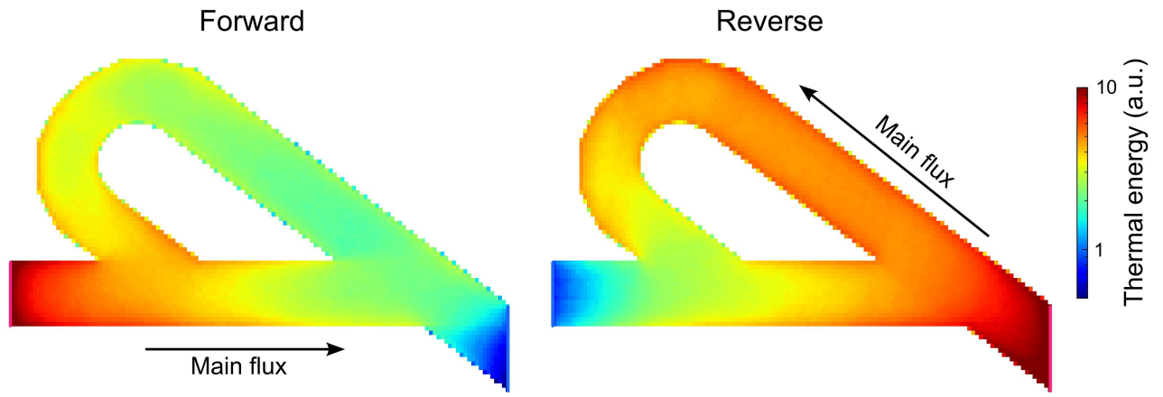
Extended Data Fig. 4 | Thermal energy maps of the Tesla valve. Thermal energy distribution in the Tesla valve in both the forward and reverse directions at 40 K using Monte Carlo simulations.
