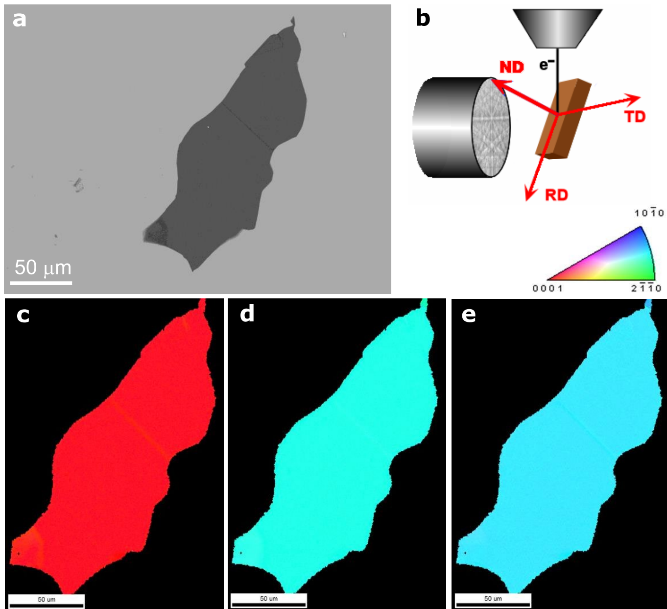
Extended Data Fig. 1 | Analysis of crystallinity by EBSD. a , Scanning electron microscopy image of the graphite sample flake used for EBSD. b , Scheme of EBSD measurement. The EBSD pattern carries information about the crystal
