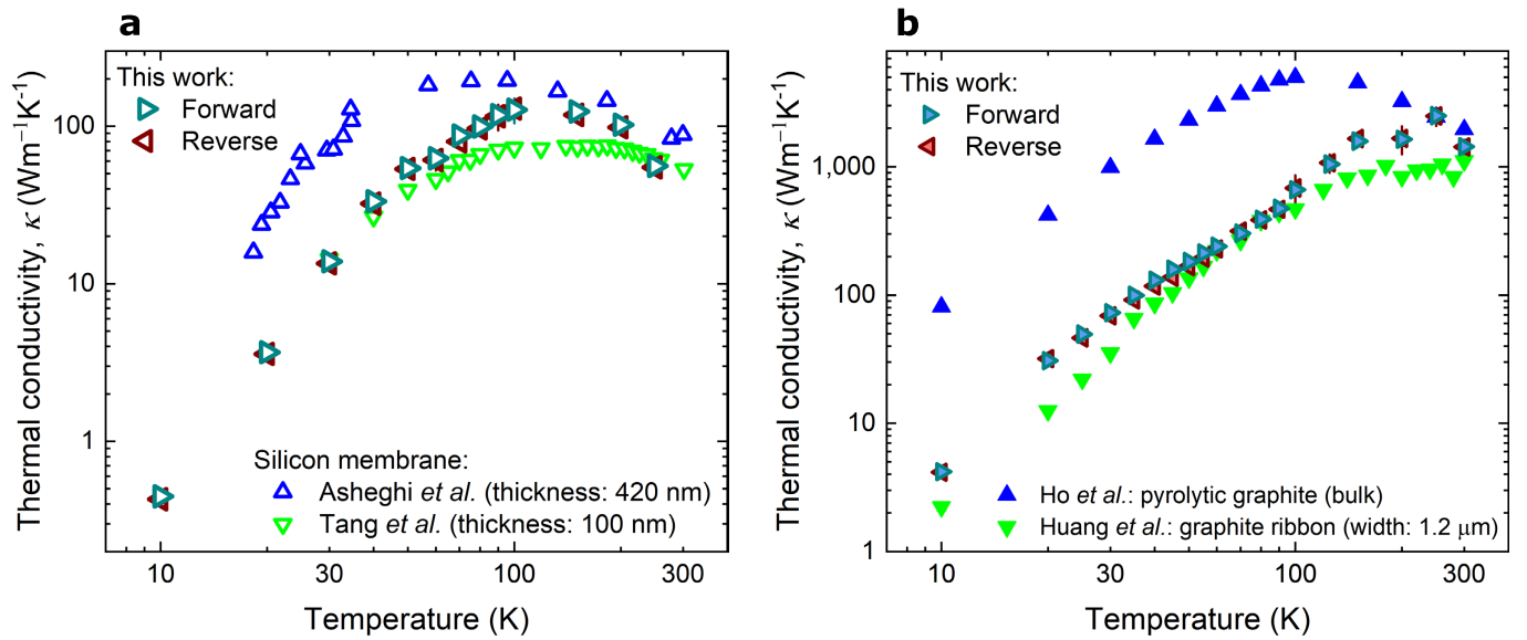
Extended Data Fig. 6 | Comparison of thermal conductivity with other literature. a , Temperature-dependent thermal conductivity of the silicon Tesla valve in the forward (open cyan triangles) and reverse (open red triangles) directions with a thickness of 145 nm (this work) and silicon membranes with
