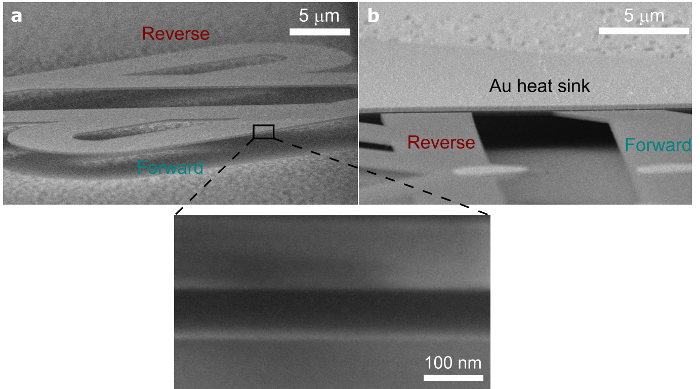
Extended Data Fig. 2 | Scanning electron microscopy images show tilted cross-section view of the samples. Suspended graphite Tesla valves vertical (a) and parallel (b) to the heat-dissipation directions.
