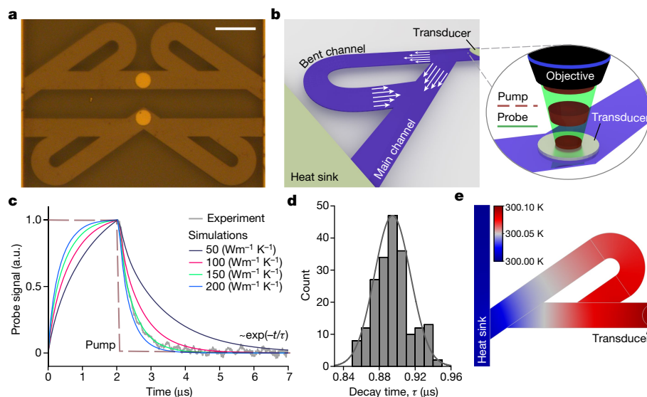
Fig. 1 | Graphite Tesla valves and thermal characterization. a , Optical microscope image of graphite Tesla valves in forward (top) and reverse (bottom) directions. Scale bar, 10 \mu\text{m} . b , Schematic of phonon hydrodynamic flows in a graphite Tesla valve in the reverse case. Arrows indicate the paths of the phonon hydrodynamic flows. Inset, schematic of the pump-probe thermoreflectance measurement. c , Example fitting of the experimental curve of the TDTR signal
