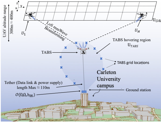
Fig. 1. System model considered around a Carleton University landscape with UAVs hovering at altitudes ranging from 300 m to 400 m.
