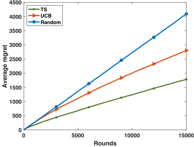
Fig. 2. The average regret plots for ten contexts for multiple training rounds using the UCB, TS, and naive-based approaches.
