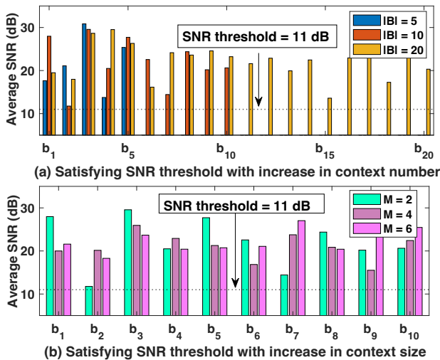
Fig. 5. Here, |B| and M represent the total number of contexts and the number of UAVs considered in the system (context size), respectively. The X axis presents context number. Each context average SNR for (a) different context numbers with fixed context size, (b) different context size with fixed context number.
