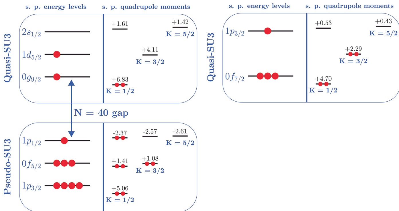
Extended Data Fig. 2 | Quasi- and Pseudo-SU3 plot for the 2p2h configuration in ^{62}\text{Cr} . Left: neutron valence space and single-particle quadrupole moments characterized by the projection of the total angular momentum on the symmetry axis, K . Right: same plot for protons. The 2p2h configuration corresponds to a
