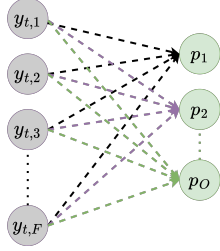
Figure 3: The fully connected layer
