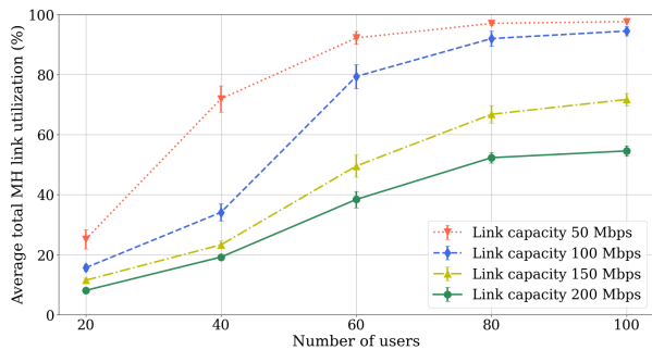
Figure 14: Average MH link utilization vs. number of users
