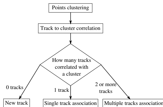
Fig. 2. Data association schema.
