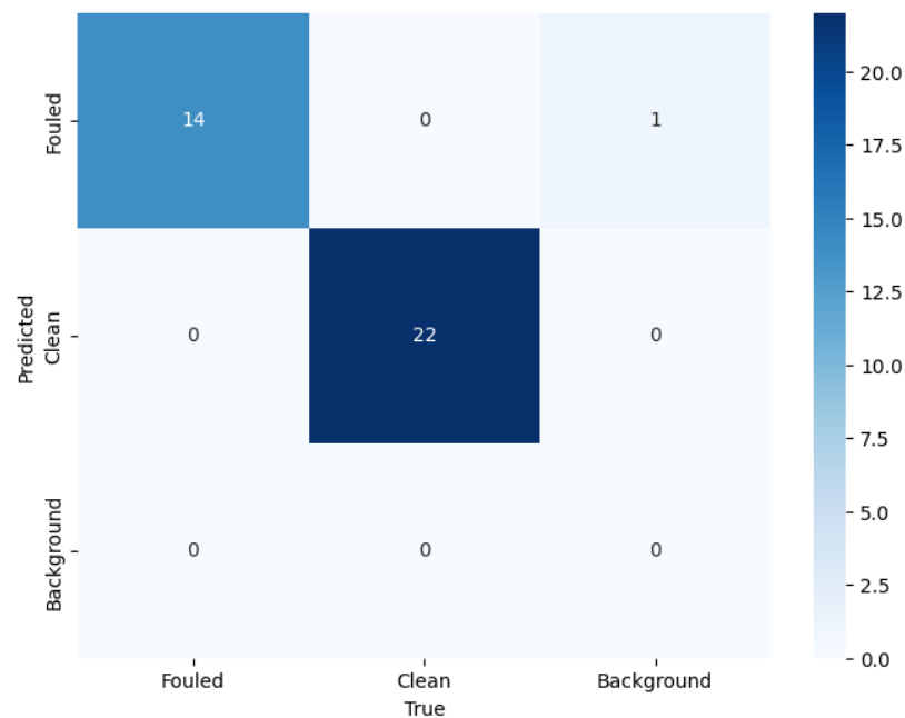
Figure 6. Confusion matrix.
